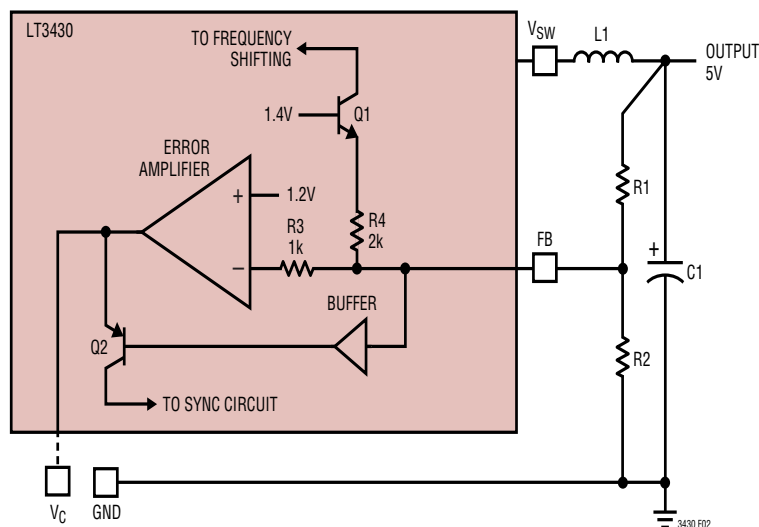
Figure 2. Frequency and Current Limit Foldback
