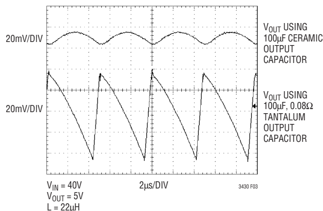
Figure 3. LT3430 Output Ripple Voltage Waveforms. Ceramic vs Tantalum Output Capacitors
