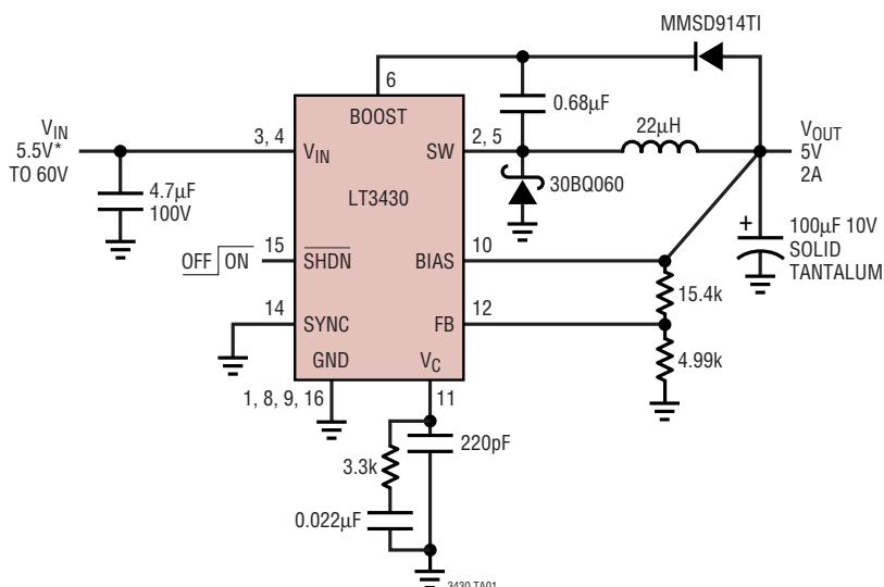
5V, 2A Buck Converter
