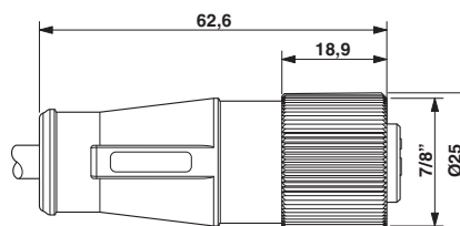
Dimensioned drawing
