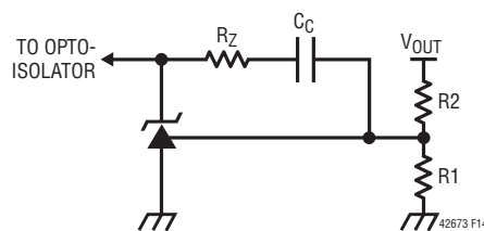
Figure 14. Main Loop Compensation for an Isolated Design
