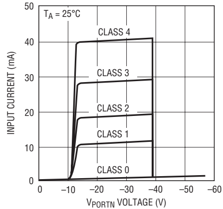
Input Current vs Input Voltage Classification Range
