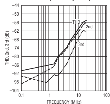
THD, 2nd and 3rd vs Input Frequency
