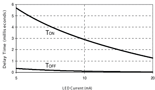
Figure 8. Typical Delay Time
