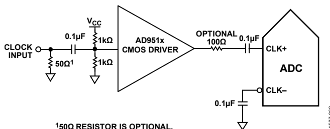
Figure 46. Single-Ended 1.8 V CMOS Input Clock (Up to 200 MHz)
