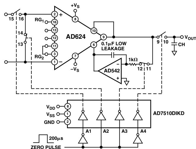
Figure 42. Autozero Circuit
