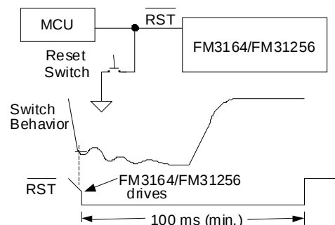
Figure 4. Manual Reset
