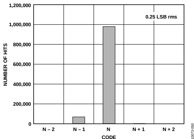
Figure 42. Input-Referred Noise Histogram, f_{\text{SAMPLE}} = 125 \text{ MSPS}
