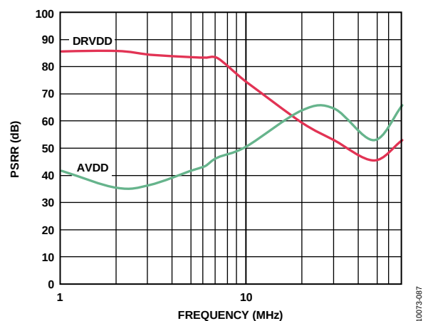
Figure 43. PSRR vs. Frequency, f_{\text{CLK}} = 125 \text{ MHz} , f_{\text{SAMPLE}} = 125 \text{ MSPS}
