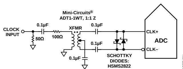
Figure 61. Transformer-Coupled Differential Clock (Up to 200 MHz)
