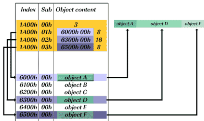
Figure 18: PDO mapping
