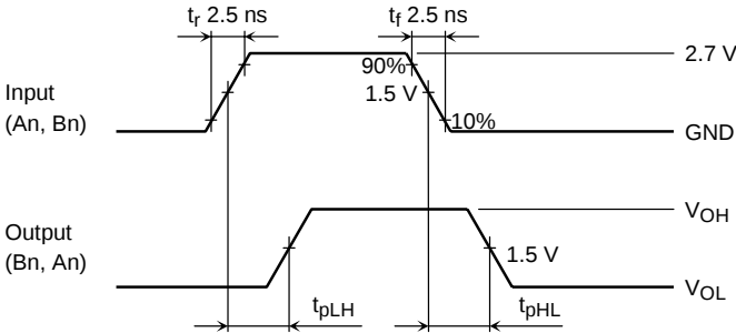
Figure 2 tpLH, tpHL
