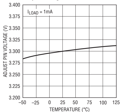
LT1129-3.3 Output Voltage
