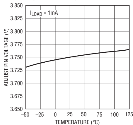
LT1129 Adjust Pin Voltage
