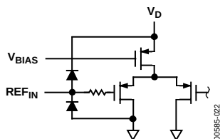
Figure 22. Equivalent Reference Input Circuit
