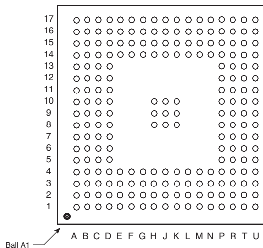
Figure 4-1. 217-ball LFBGA Package (Top View)
