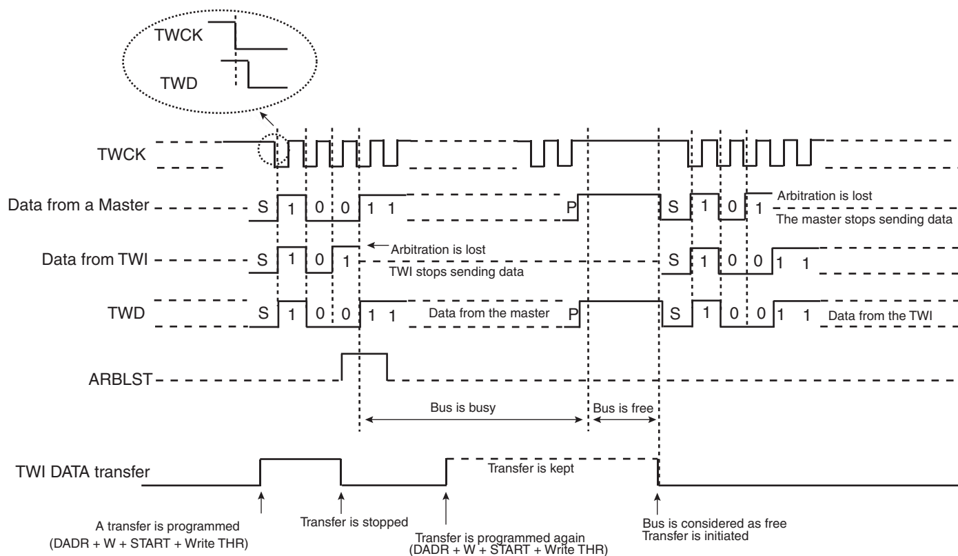
Figure 31-21. Arbitration Cases
