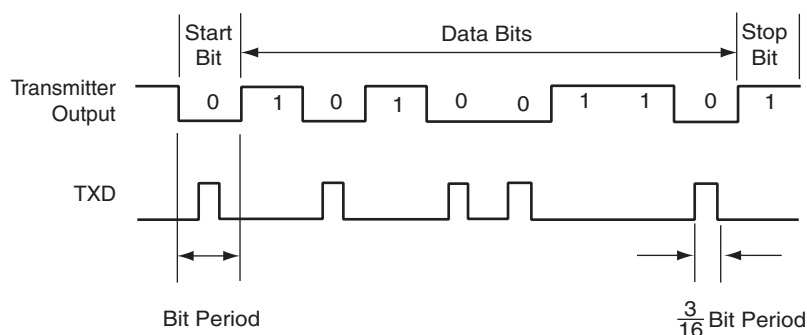
Figure 32-34. IrDA Modulation
