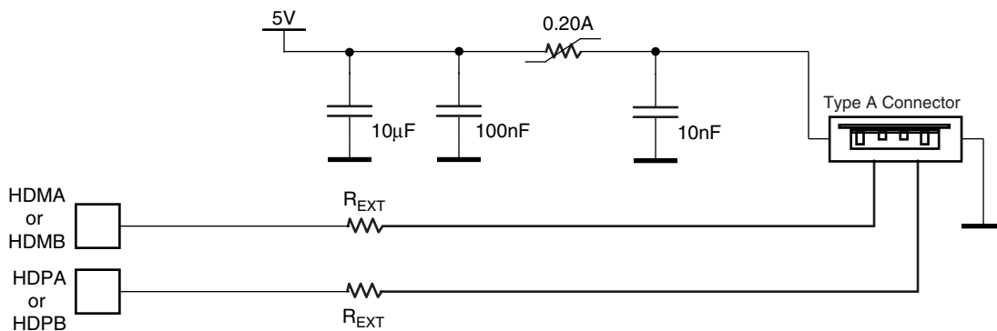
Figure 38-4. Board Schematic to Interface UHP Device Controller
