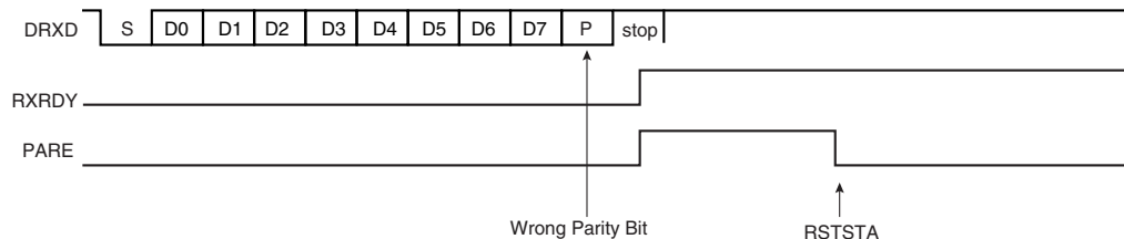
Figure 28-9. Parity Error
