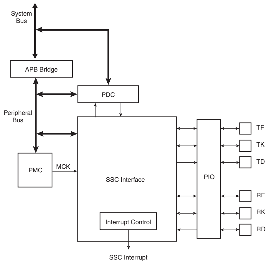
Figure 33-1. Block Diagram
