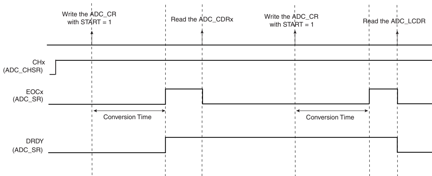
Figure 40-2. EOCx and DRDY Flag Behavior
