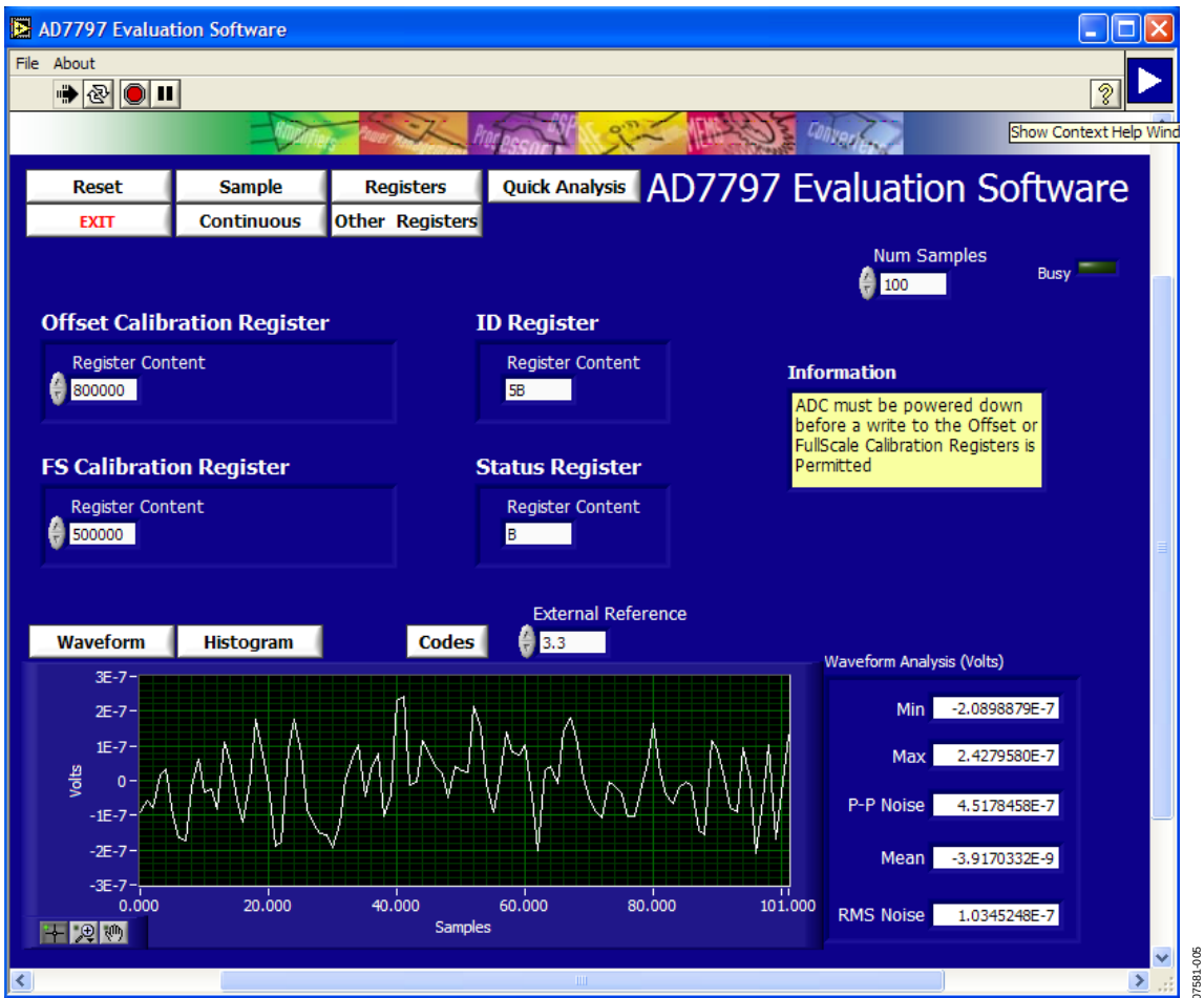
Figure 5. AD7797 Evaluation Software Other Registers Window
