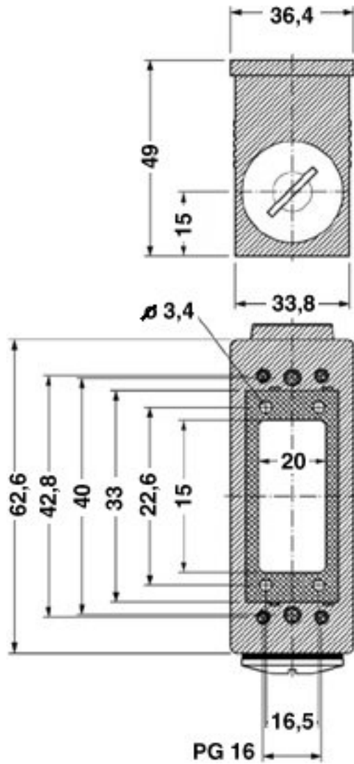
Dimensioned drawing
