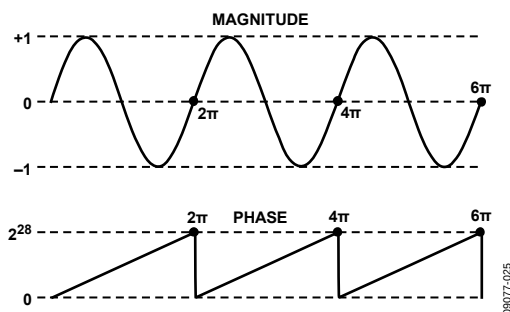
Figure 20. Sine Wave
