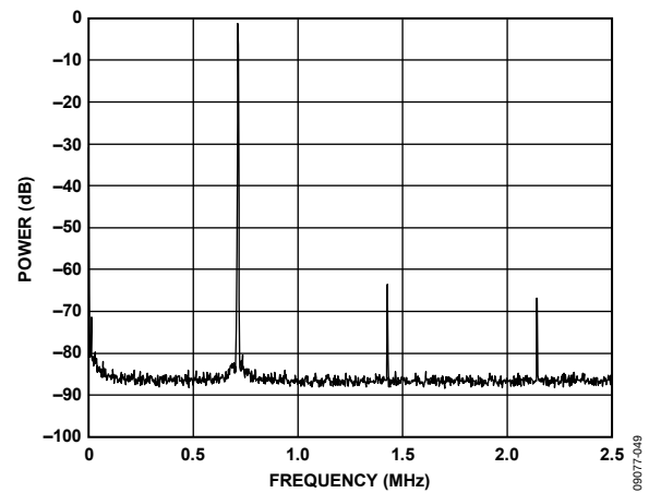
Figure 17. Power vs. Frequency, f_{CLK} = 5\text{ MHz} , f_{OUT} = 0.714\text{ MHz} = f_{CLK}/7 , Frequency Word = 0x2492492
