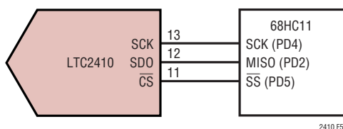
Figure 55. Connecting the LTC2410 to a 68HC11 MCU Using the SPI Serial Interface
