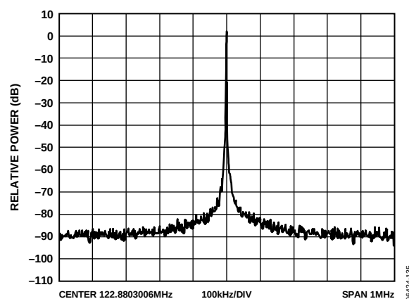
Figure 17. Output Spectrum, LVPECL; 122.88 MHz; PFD = 15.36 MHz; LBW = 190 kHz; I_{CP} = 4.2 \text{ mA} ; f_{VCO} = 2.7 \text{ GHz}
