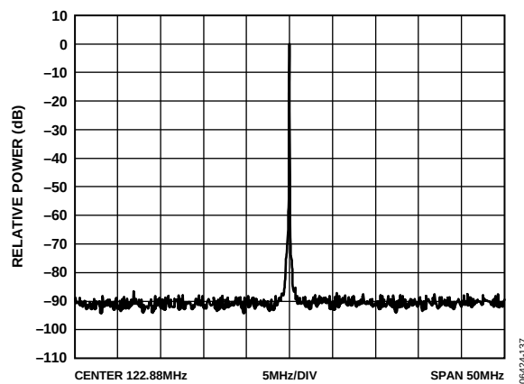
Figure 16. PFD/CP Spurs; 122.88 MHz; PFD = 15.36 MHz; LBW = 190 kHz; I_{CP} = 4.2 \text{ mA} ; f_{VCO} = 2.7 \text{ GHz}
