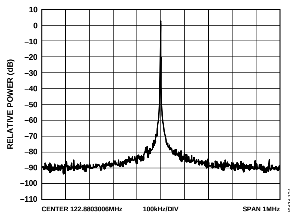
Figure 18. Output Spectrum, LVDS; 122.88 MHz; PFD = 15.36 MHz; LBW = 190 kHz; I_{CP} = 4.2 \text{ mA} ; f_{VCO} = 2.7 \text{ GHz}
