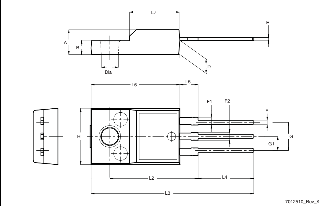
Figure 23. TO-220FP drawing
