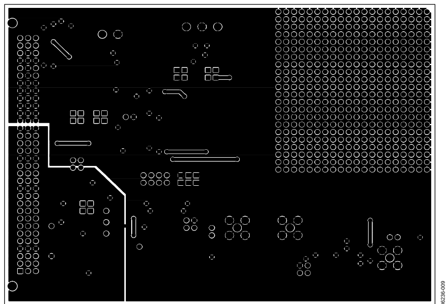
Figure 9. Solder Side Artwork
