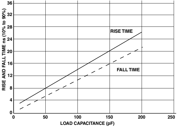
Figure 62. Typical Output Delay or Hold for Driver F at V_{DDEXT} \text{ Max}
