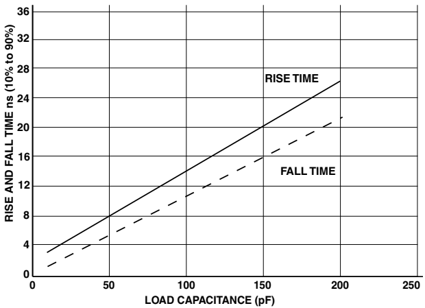
Figure 61. Typical Output Delay or Hold for Driver F at V_{DDEXT} \text{ Min}
