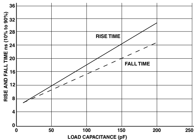
Figure 59. Typical Output Delay or Hold for Driver E at V_{DDEXT} \text{ Min}
