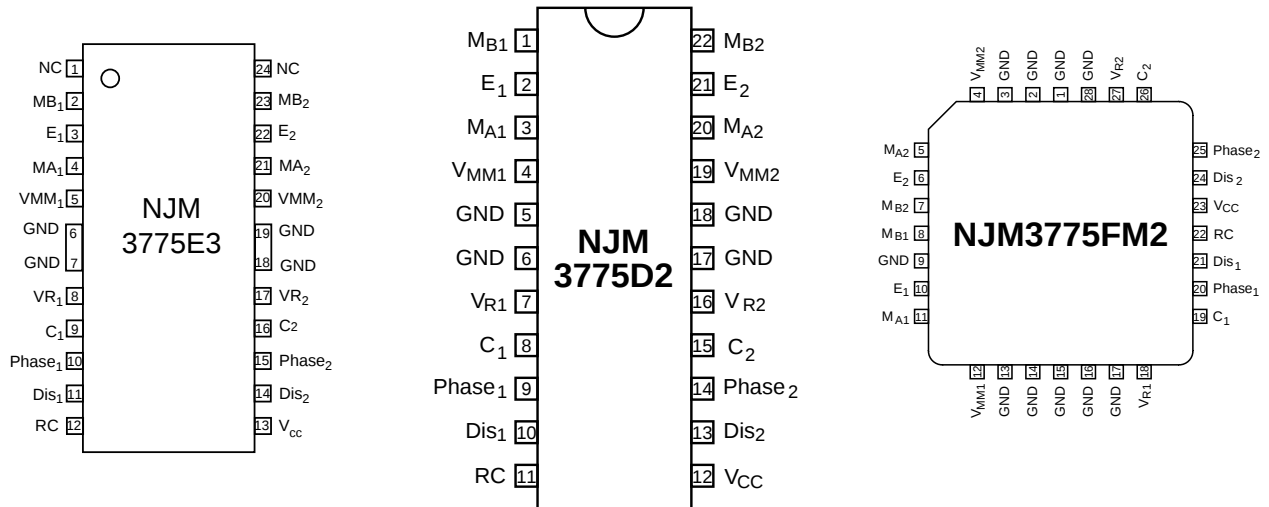
Figure 2. Pin configurations
