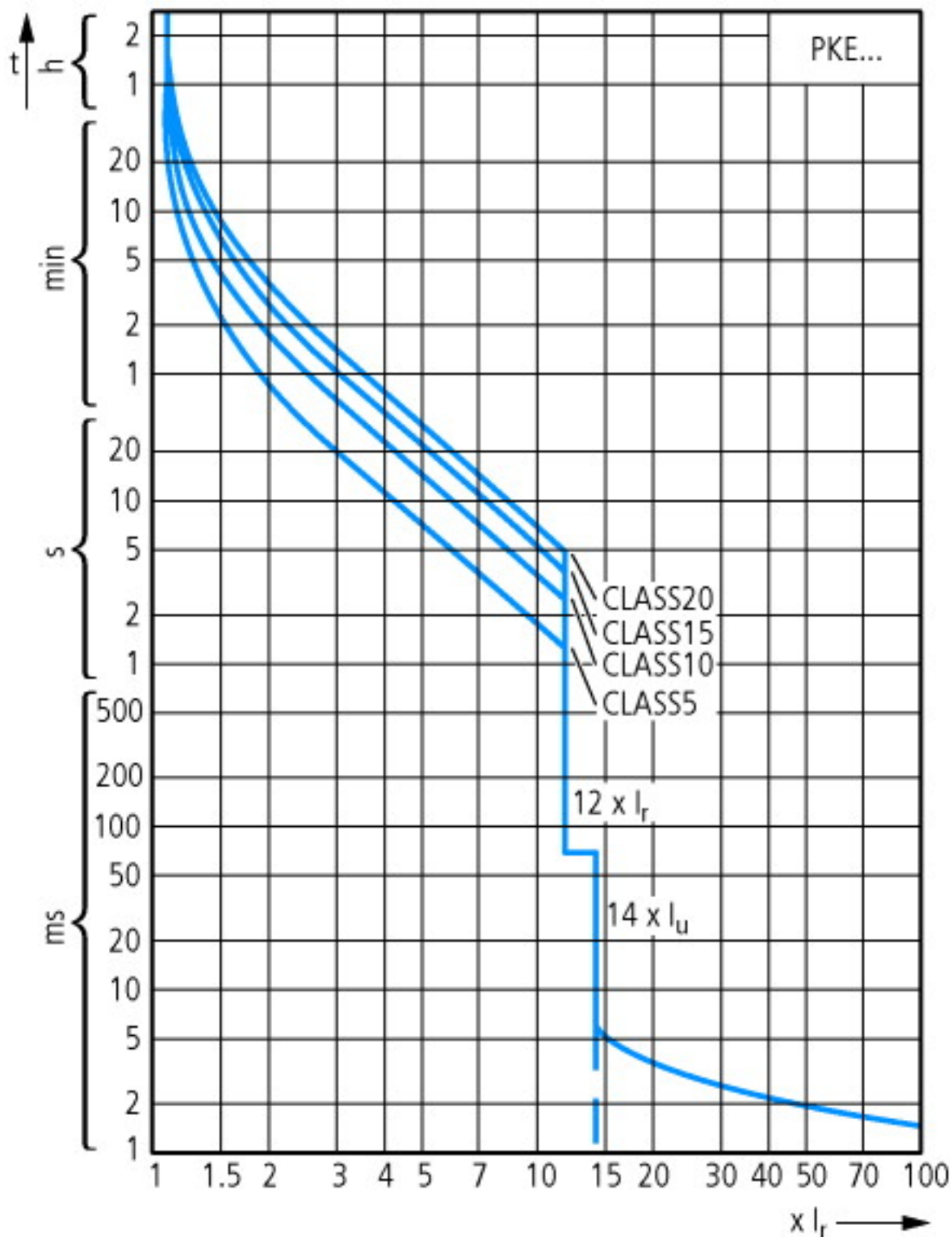
Tripping characteristics
