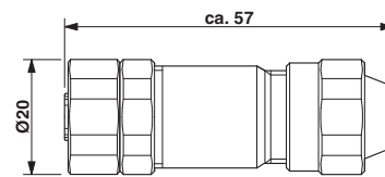
M12 x 1 socket, straight, shielded
