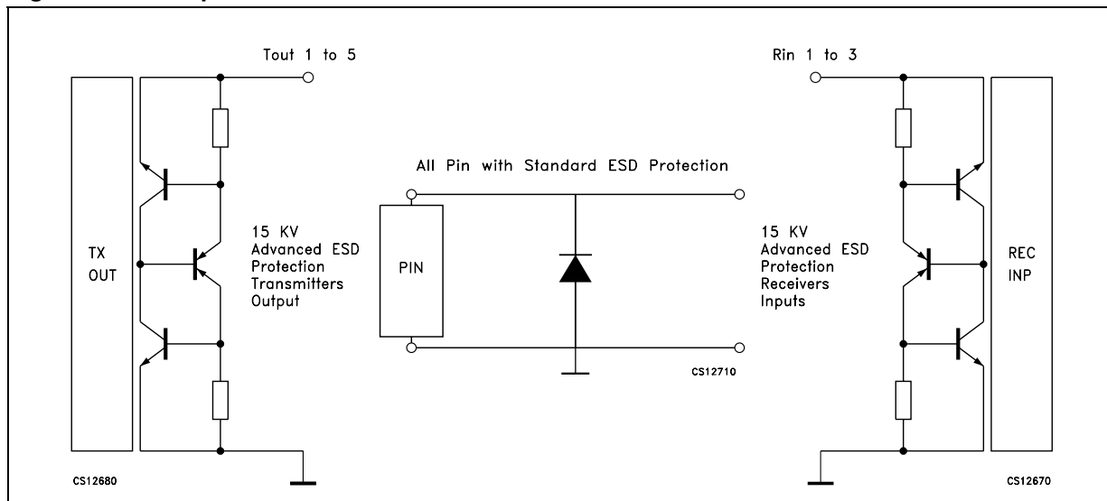
Figure 6. ESD protection
