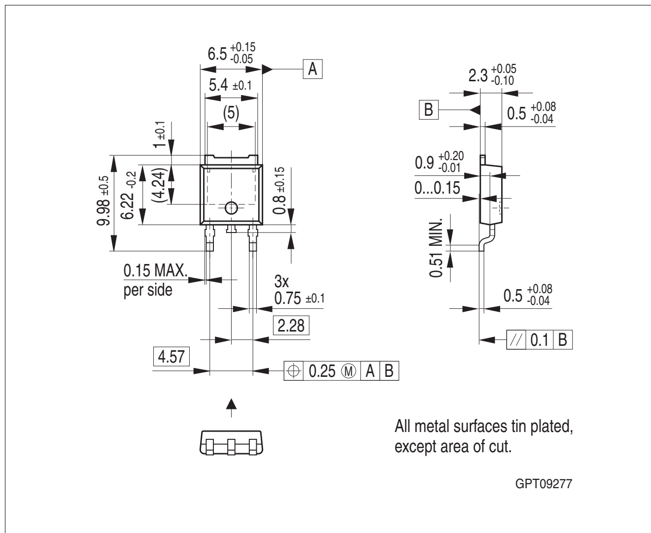
Figure 5 PG-TO252-3
