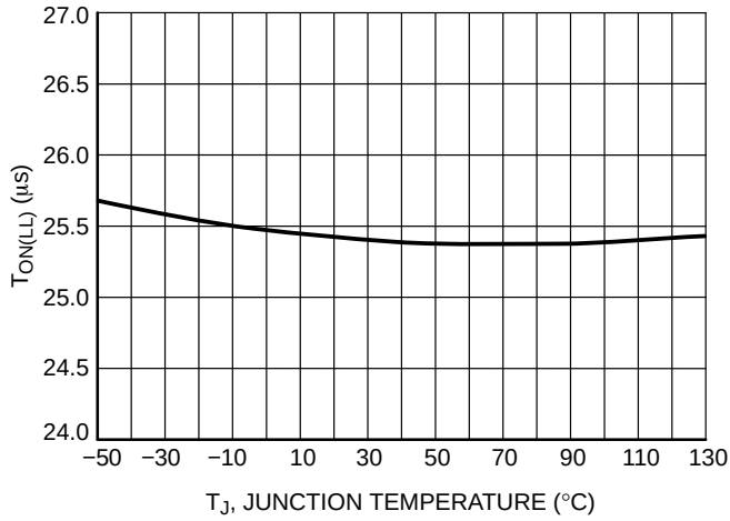
Figure 40. Maximum On Time @ V_{SENSE} = 1.4 V vs. Temperature
