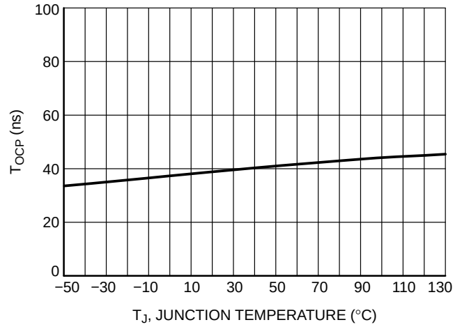
Figure 29. Over-current Protection Delay from V_{CS/ZCD} > V_{CS(th)} to DRV Low ( dV_{CS/ZCD} / dt = 10 \text{ V}/\mu\text{s} ) vs. Temperature
