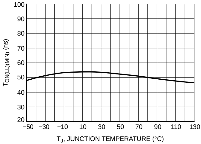
Figure 42. Minimum On Time @ V_{SENSE} = 1.4 V vs. Temperature
