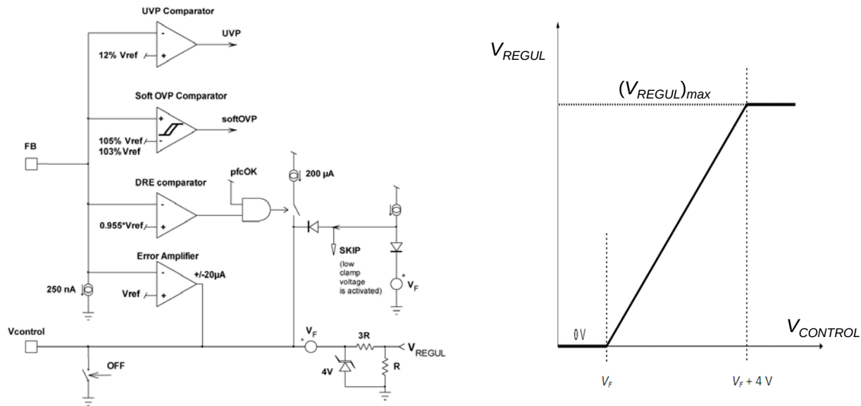
Figure 68. a) Regulation Block Figure (left), b) Correspondence between V_{\text{CONTROL}} and V_{\text{REGUL}} (right)
