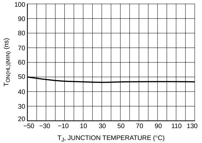
Figure 43. Minimum On Time @ V_{SENSE} = 2.8 V vs. Temperature
