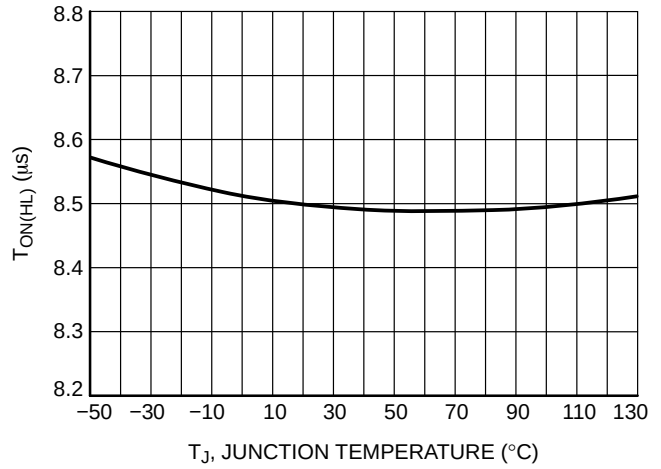
Figure 41. Maximum On Time @ V_{SENSE} = 2.8 V vs. Temperature
