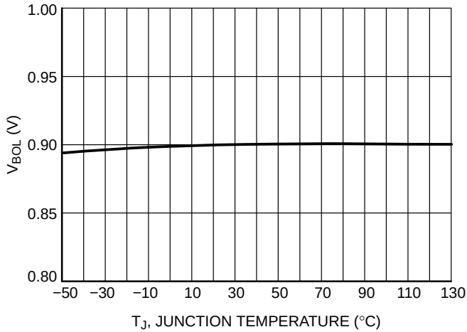
Figure 52. Brown-out Threshold, V_{SENSE} Falling vs. Temperature
