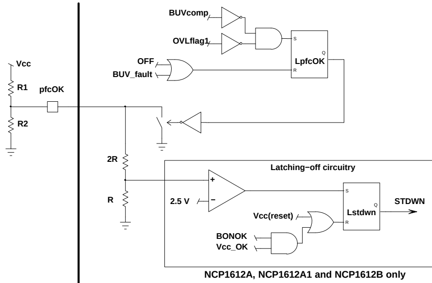
Figure 71. pfcOK Detection
