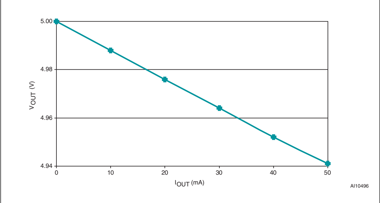
Figure 19. Output voltage vs. load current ( V_{\text{CC}} = 5\text{ V} ; T_{\text{A}} = 25\text{ °C} )
