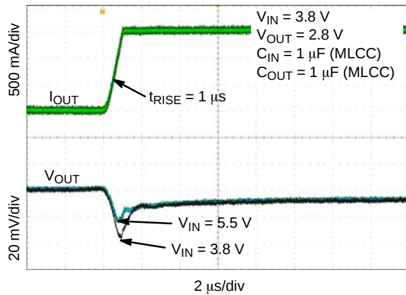
Figure 38. Load Transient Response – Rising Edge, V_{OUT} = 2.8 V , I_{OUT} = 1 mA to 150 mA, V_{IN} = 3.8 V , 5.5 V
