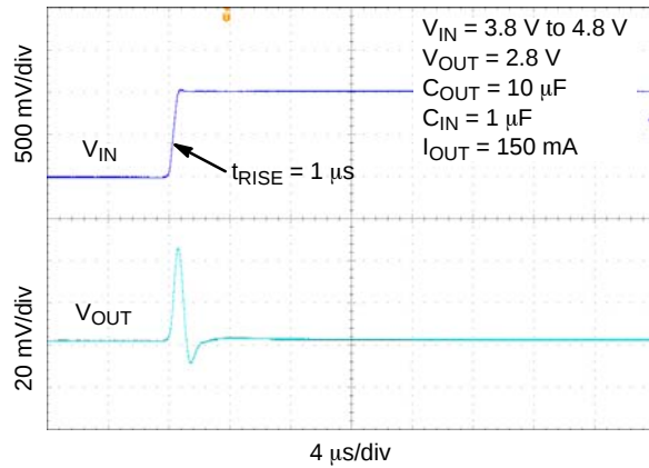
Figure 32. Line Transient Response – Rising Edge, V_{OUT} = 2.8 \text{ V} , I_{OUT} = 150 \text{ mA}
