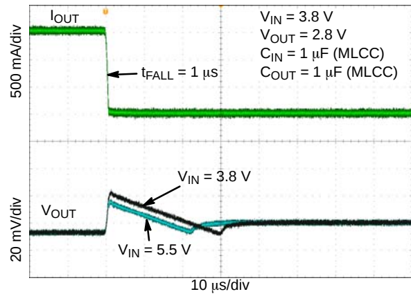
Figure 39. Load Transient Response – Falling Edge, V_{OUT} = 2.8 V , I_{OUT} = 1 mA to 150 mA, V_{IN} = 3.8 V , 5.5 V
