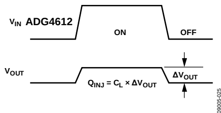
Figure 27. Charge Injection
