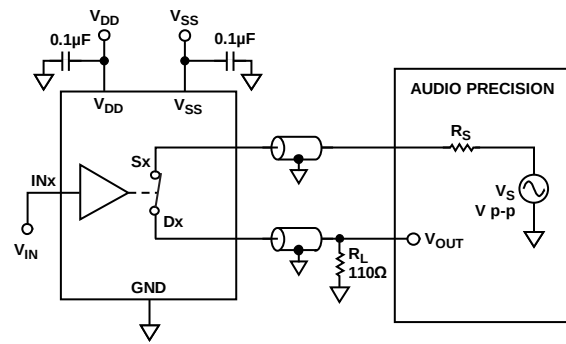
Figure 31. THD + Noise
