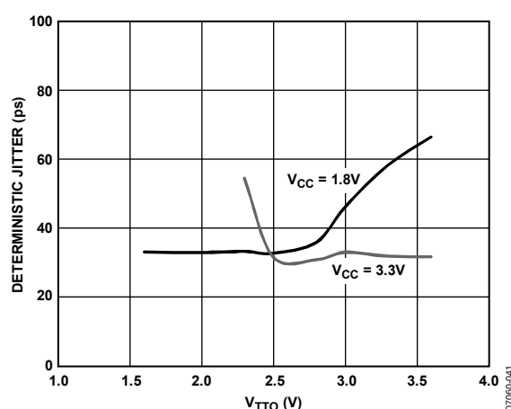
Figure 35. Deterministic Jitter vs. Output Termination Voltage (V TT0 )
