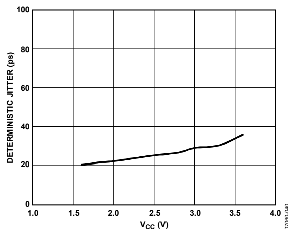
Figure 34. Deterministic Jitter vs. Supply Voltage (V CC )
