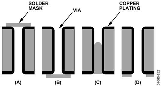
Figure 48. Solder Mask Options for Thermal Vias: (a) Via Tenting from the Top; (b) Via Tenting from the Bottom; (c) Via Plugging, Bottom; and (d) Via Encroaching, Bottom
