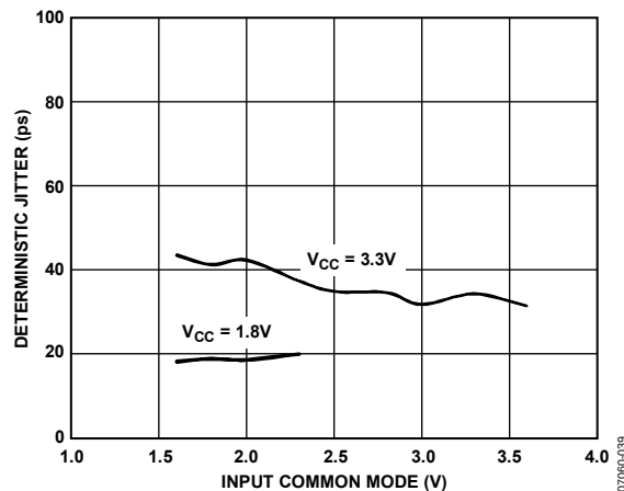
Figure 33. Deterministic Jitter vs. Input Common Mode
