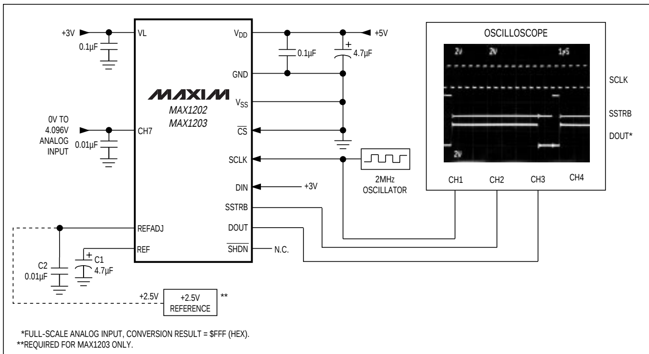
Figure 5. Quick-Look Circuit
