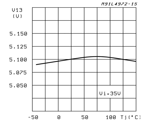
Figure 20. Reference Voltage (pin 13) vs. Junction Temperature (see fig. 11).
