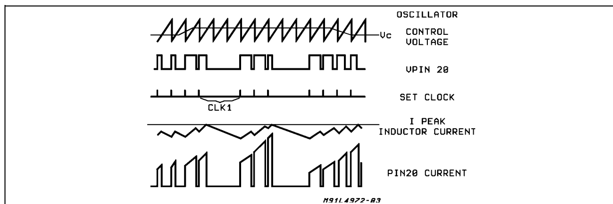
Figure 6. Limiting Current Function.
