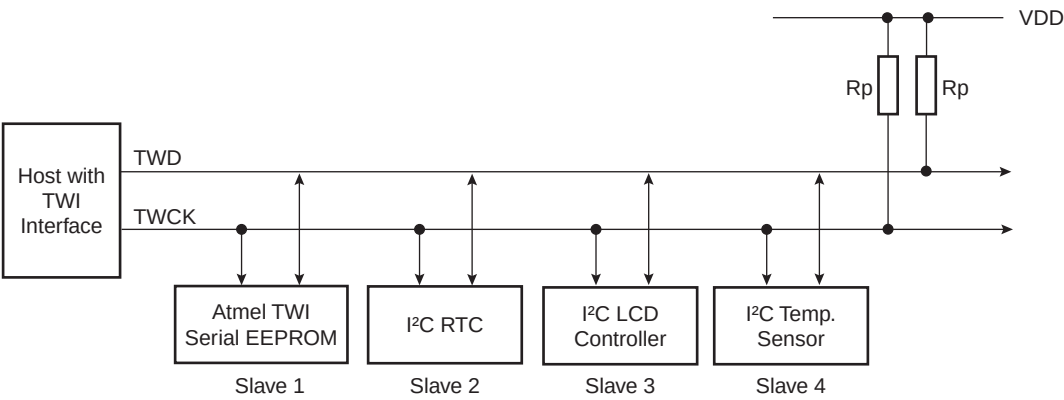
Figure 32-2. Application Block Diagram
