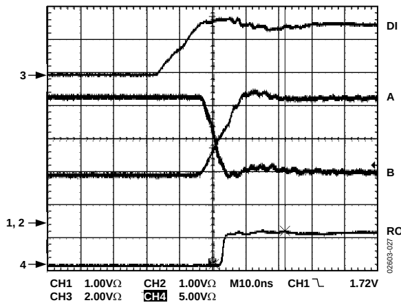
Figure 27. Driver/Receiver Propagation Delays Low to High ( R_{L\text{Diff}} = 54 \Omega , C_{L1} = C_{L2} = 100 \text{ pF} )
