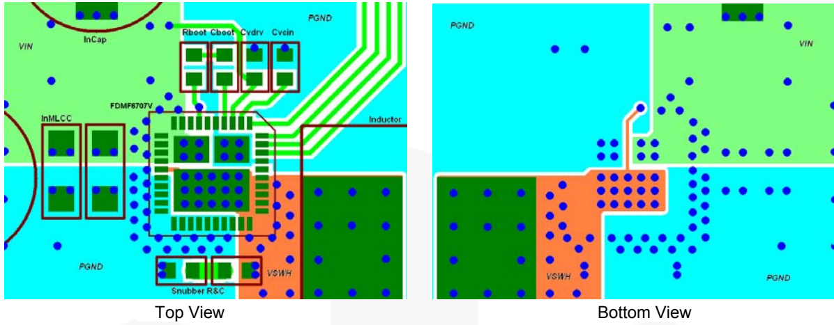
Figure 28. PCB Layout Example
