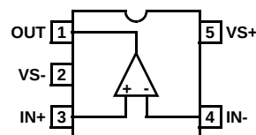
EL5167 (5 LD SOT-23, SC-70) TOP VIEW
