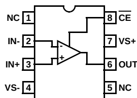
EL5166 (8 LD SOIC) TOP VIEW
