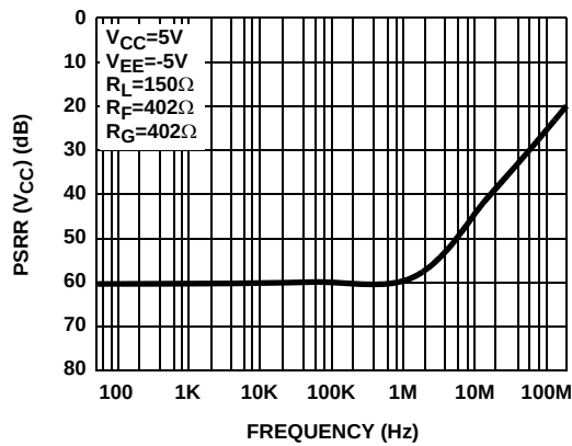
FIGURE 11. PSRR +5V
