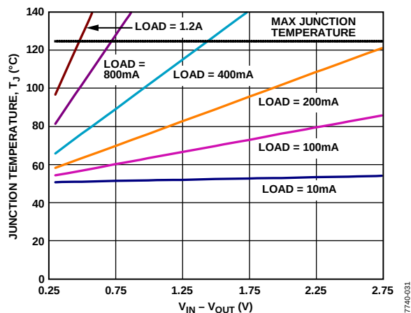
Figure 16. 0 mm 2 of PCB Copper, T_A = 50^\circ\text{C} , LFCSP
