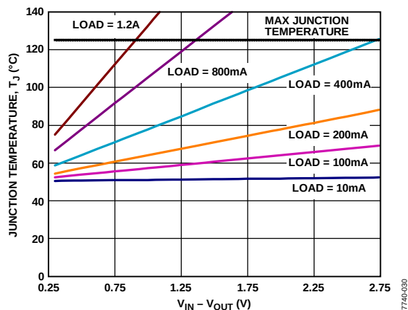
Figure 15. 500 mm 2 of PCB Copper, T_A = 50^\circ\text{C} , LFCSP
