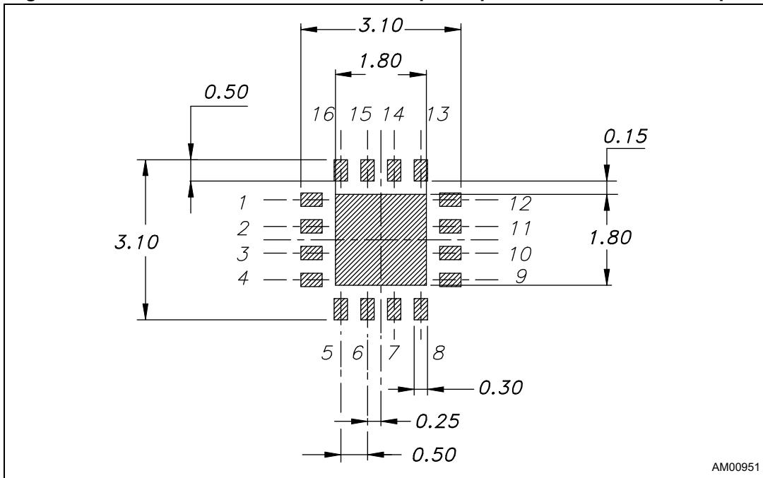
Figure 26. VFQFPN 16L 3 x 3 x 0.8 mm with exposed pad 1.7 recommended footprint
