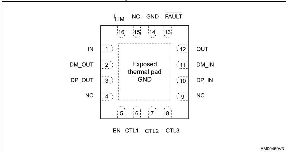
Figure 2. Pinout
