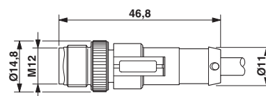
Dimensioned drawing
