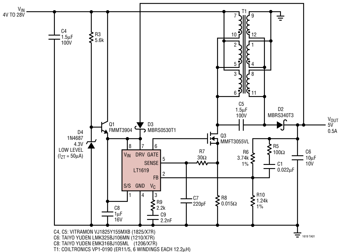
Figure 19. 2.5W, 4V IN -28V IN to 5V/0.5A Nonisolated Supply
