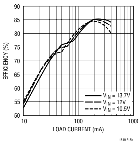
Figure 18b. Efficiency of the Isolated Local SLIC (Flyback)
