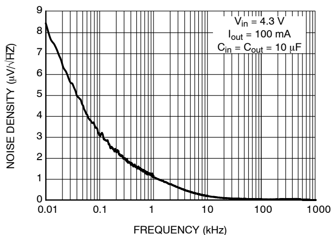
Figure 24. Output Noise density vs. Frequency at NCP4632xDT33
