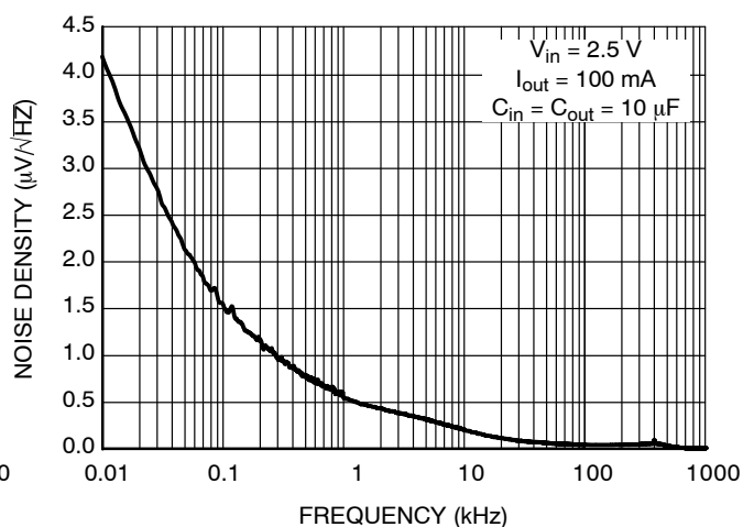
Figure 22. Output Noise Density vs. Frequency at NCP4632xDT15
