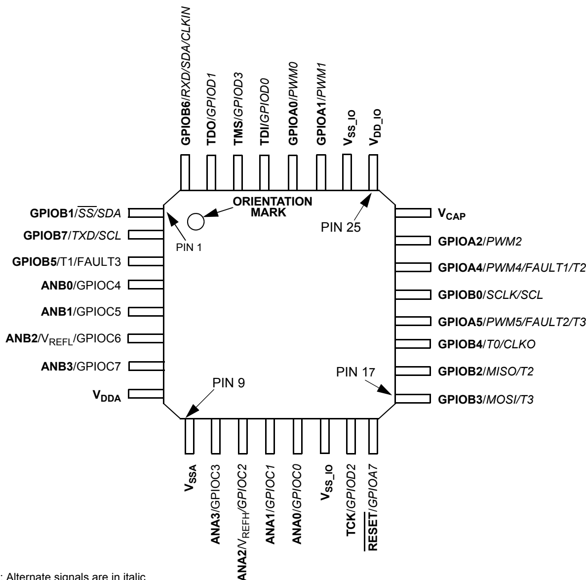
Figure 11-1 Top View, 56F8014 32-Pin LQFP Package
