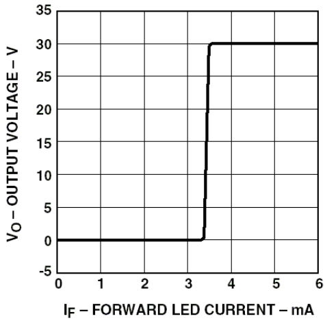
Figure 13. Transfer characteristics.
