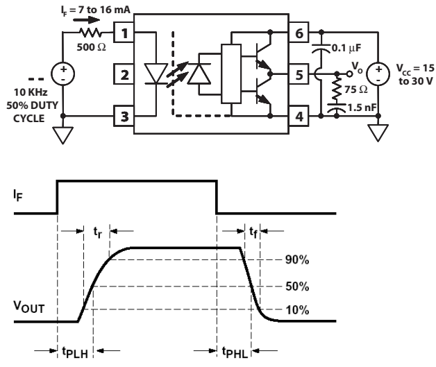
Figure 15. Propagation Delay Test Circuit and Waveforms.
