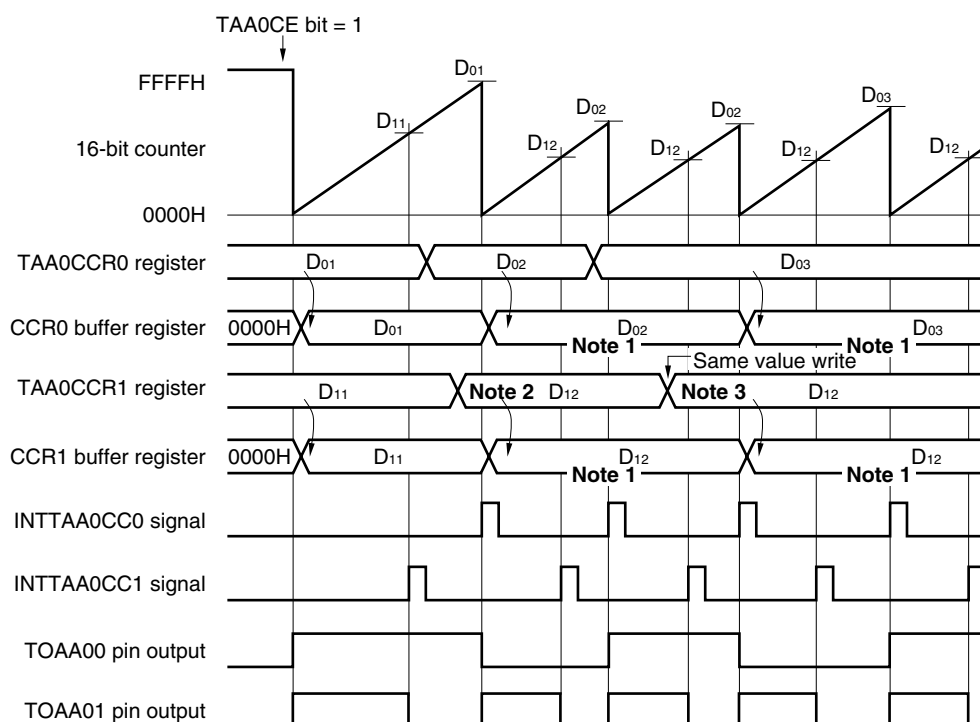
Figure 6-6. Timing of Batch Write (Interval Timer Mode of TAA0)
