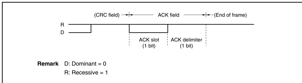
Figure 19-11. ACK Field
