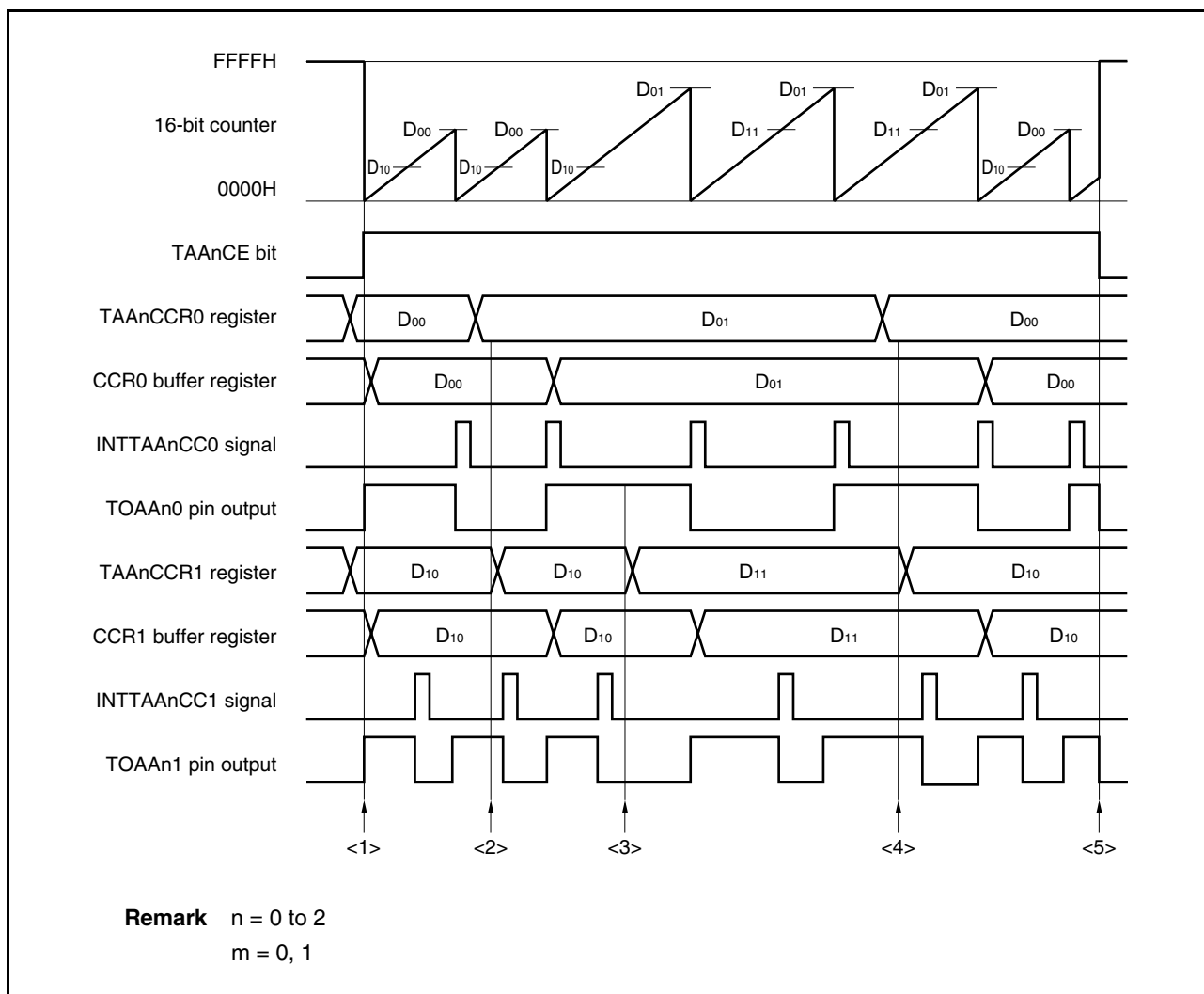
Figure 6-32. Software Processing Flow in PWM Output Mode (1/2)
