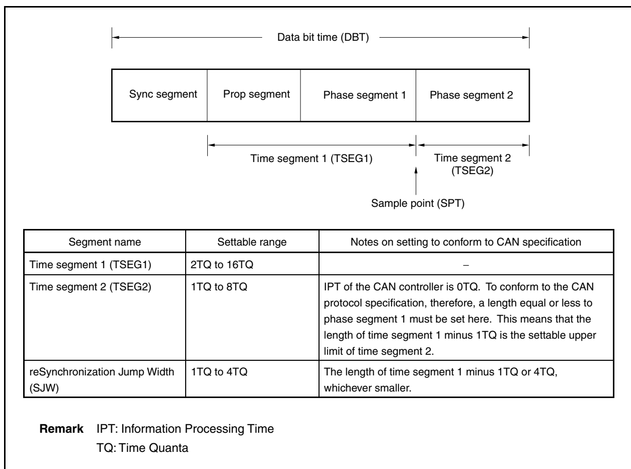
Figure 19-18. Segment Setting
