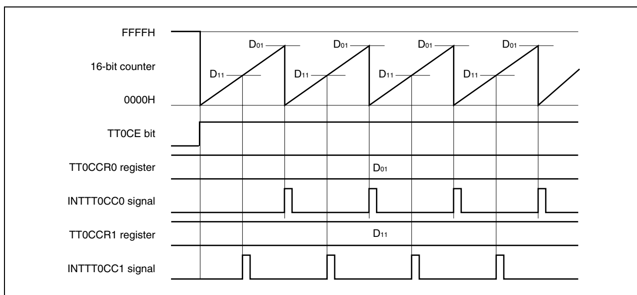
Figure 8-19. Timing Chart When D_{01} \geq D_{11}
