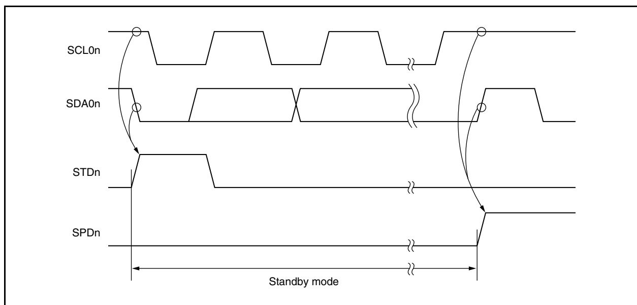
Figure 18-16. Timing for Accepting Communication Reservations
