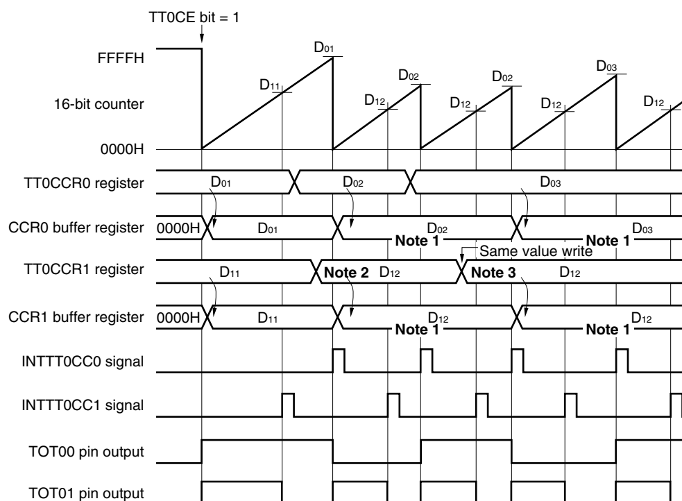
Figure 8-6. Timing of Batch Write
