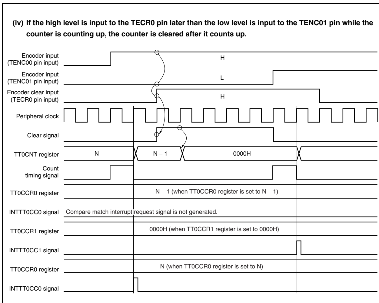
Figure 8-54. Operation Example (When TT0SCE Bit = 1, TT0ZCL Bit = 1, TT0BCL Bit = 0, TT0ACL Bit = 1, TT0UDS1 and TT0UDS0 Bits = 11, TECR0 = High Level, TENC01 = Low Level, and TENC00 = High Level) (3/3)
