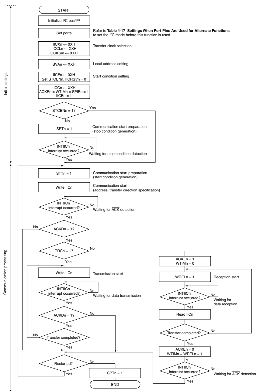
Figure 18-18. Master Operation in Single Master System
