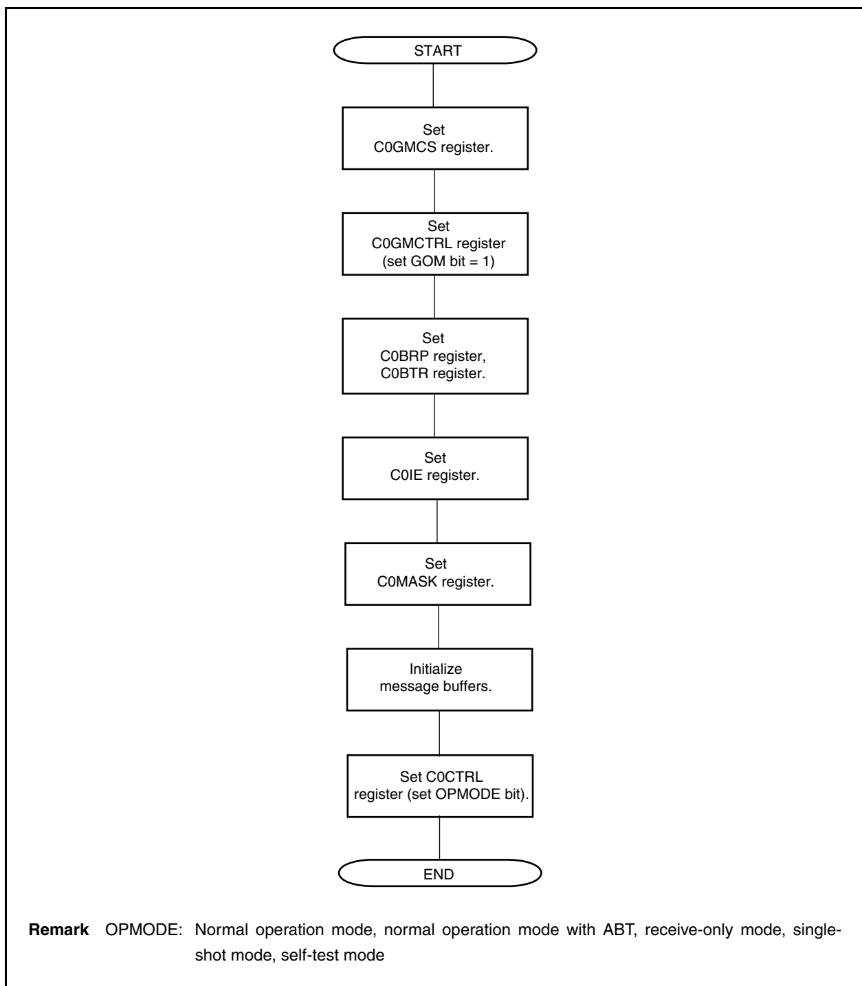
Figure 19-36. Initialization
