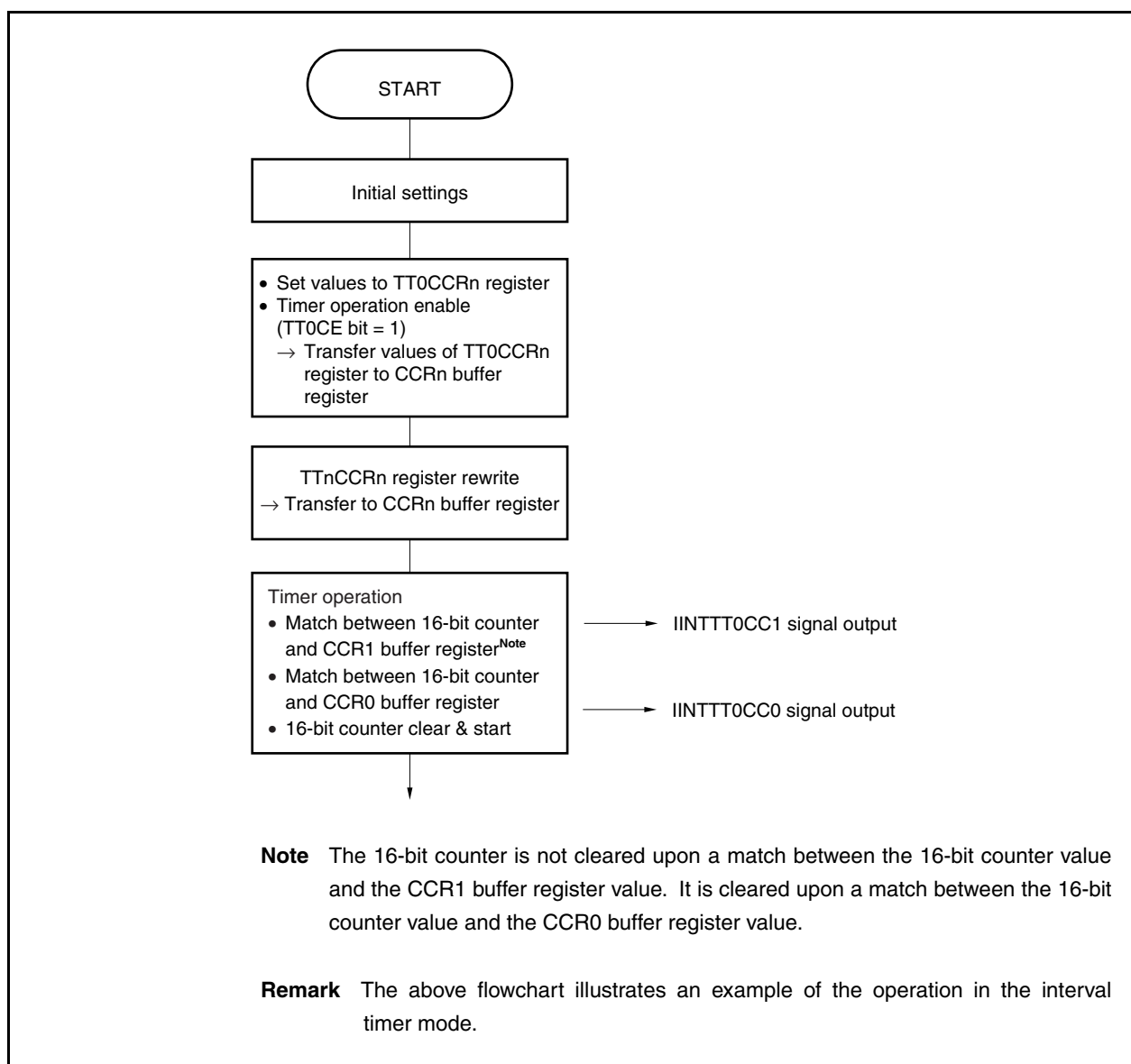
Figure 8-3. Flowchart of Basic Operation for Anytime Write
