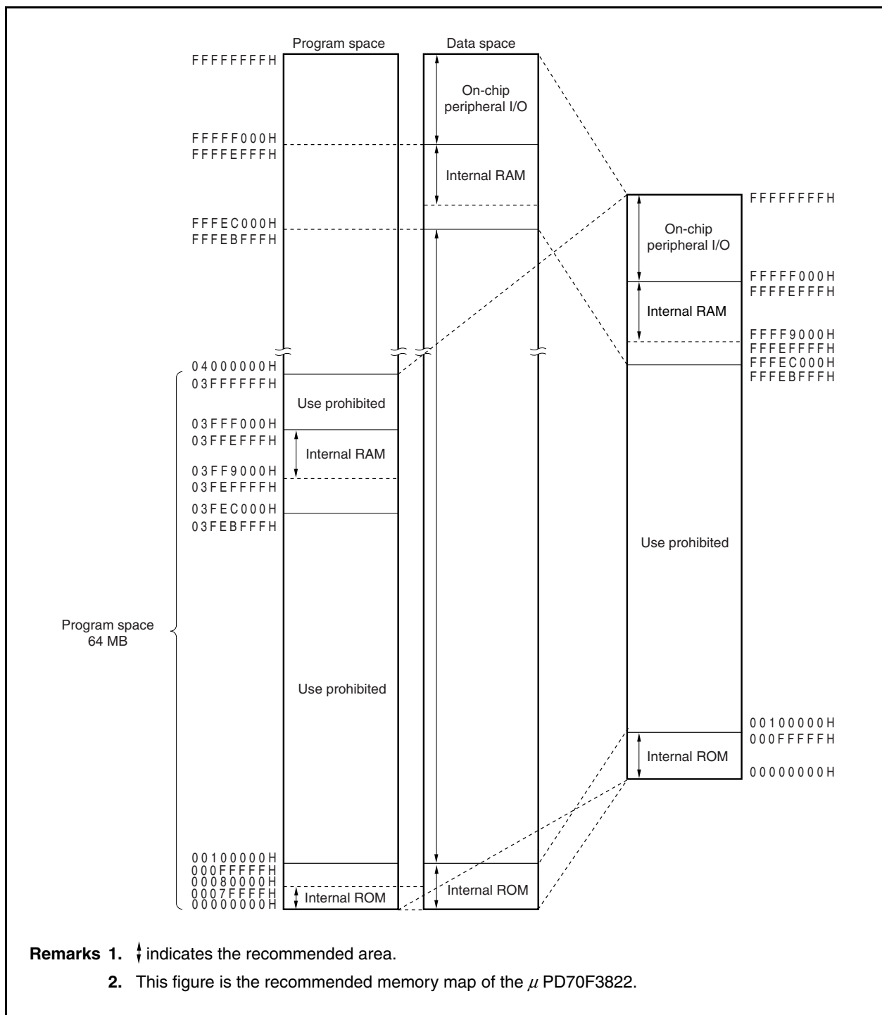
Figure 3-14. Recommended Memory Map
