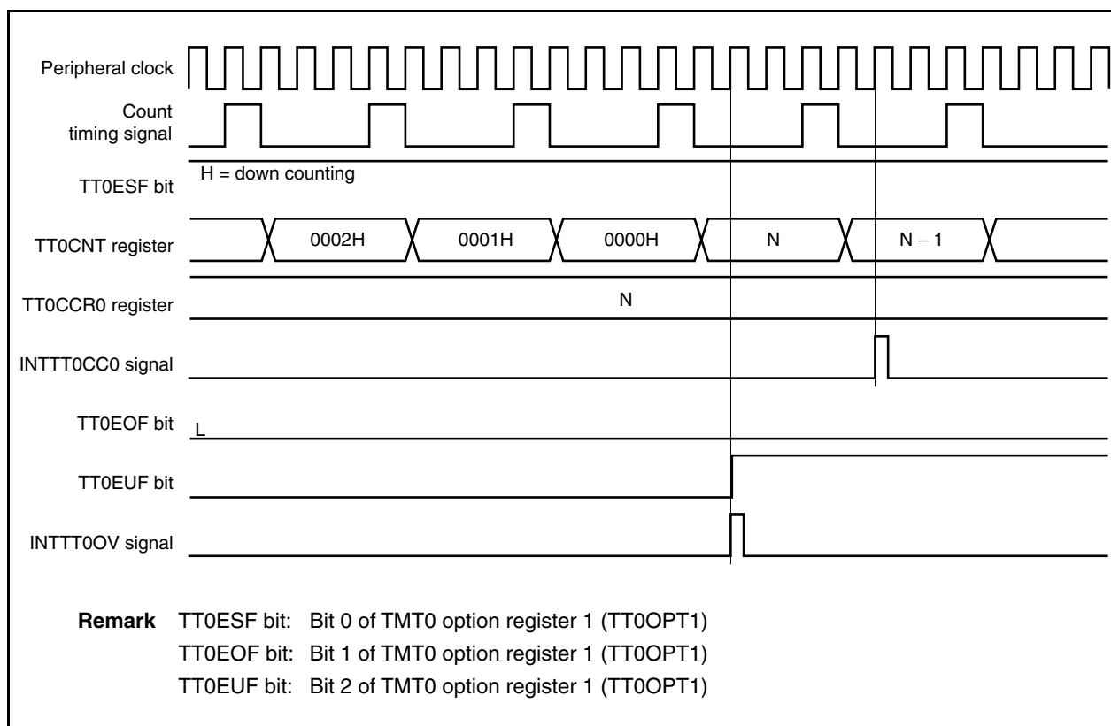
Figure 8-52. Operation Timing (Count Operation in Range from 0000H to Set Value of TT0CCR0 Register)
