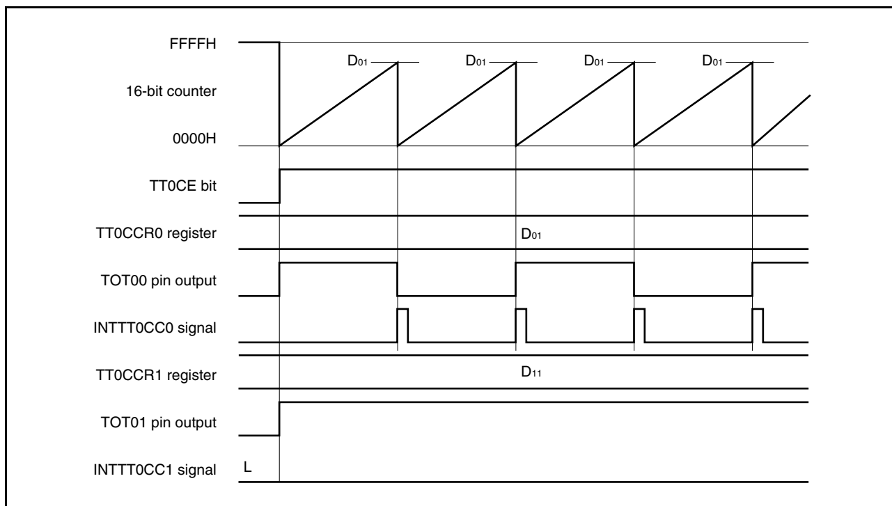
Figure 8-13. Timing Chart When D_{01} < D_{11}
