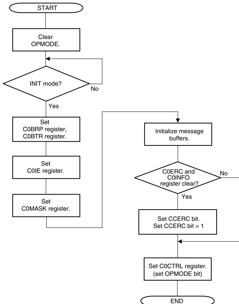
Figure 19-37. Re-initialization
