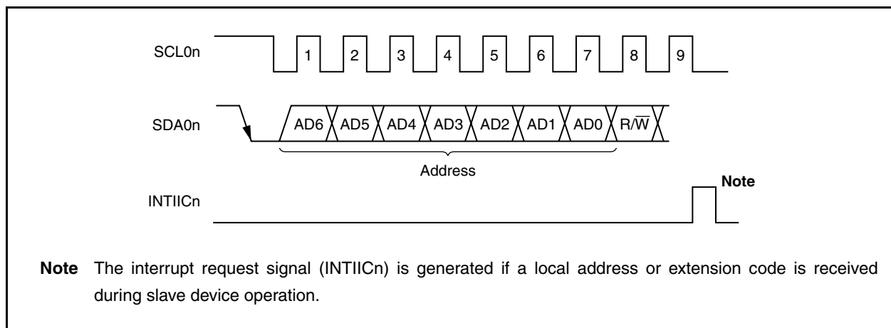
Figure 18-9. Address
