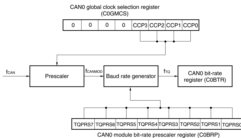
Figure 19-23. CAN Module Clock
