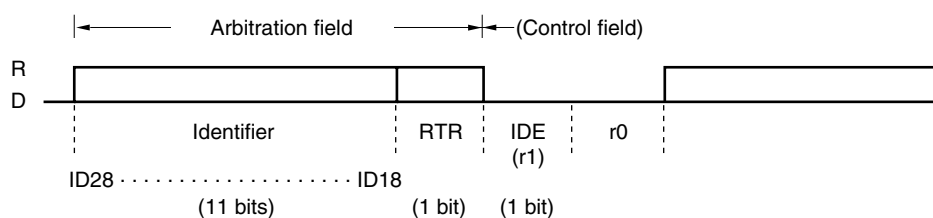
Figure 19-6. Arbitration Field (in Standard Format Mode)
