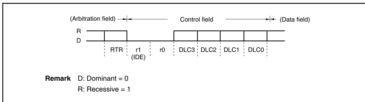
Figure 19-8. Control Field
