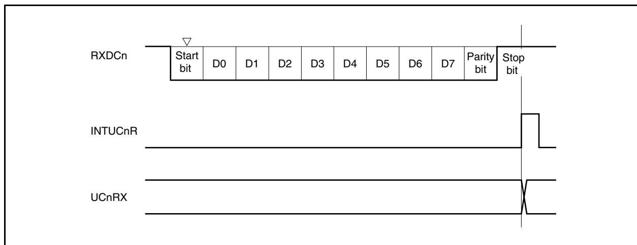
Figure 16-14. UART Reception
