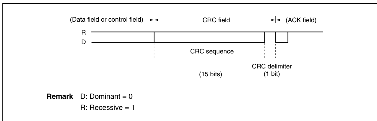
Figure 19-10. CRC Field
