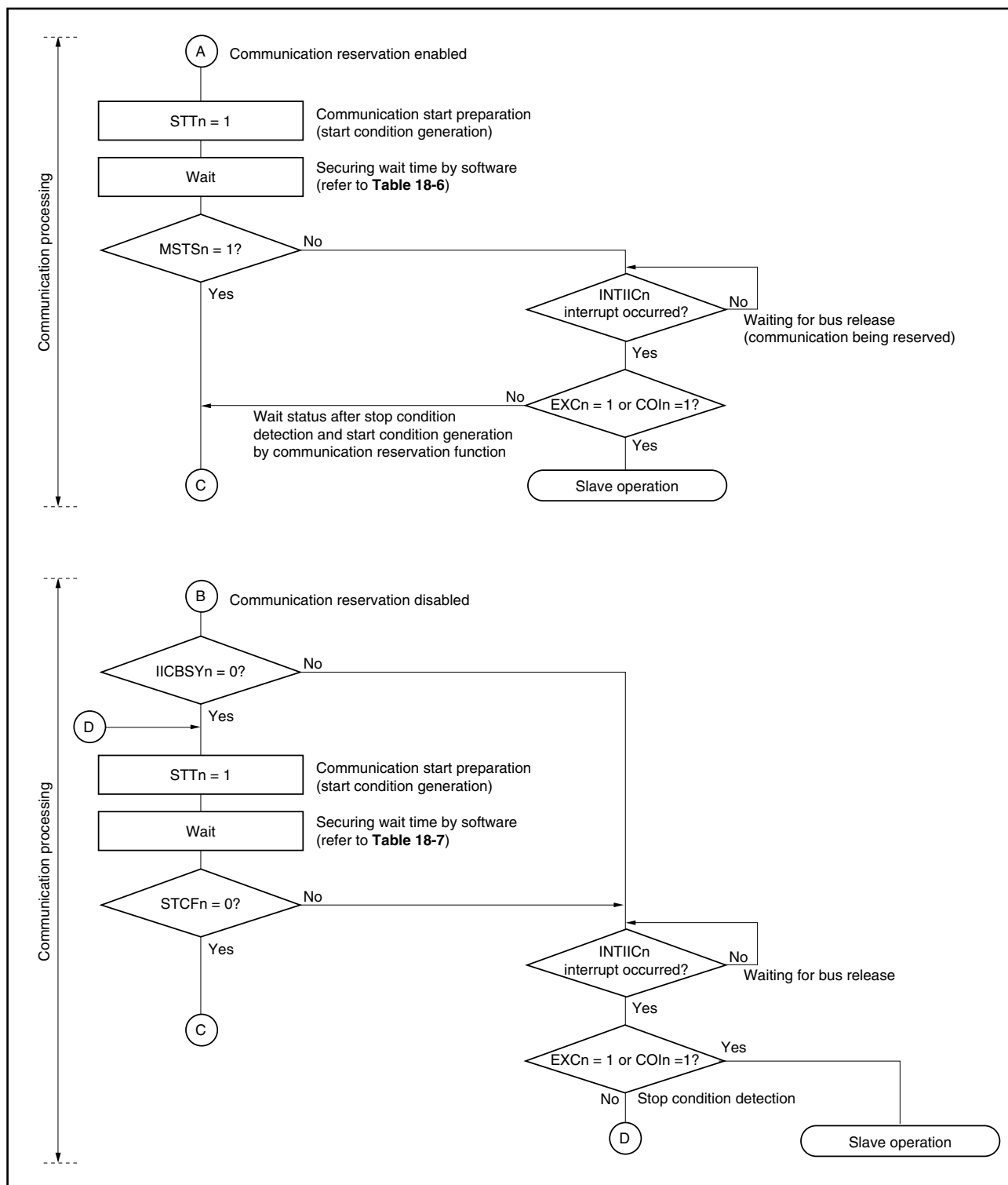
Figure 18-19. Master Operation in Multimaster System (2/3)
