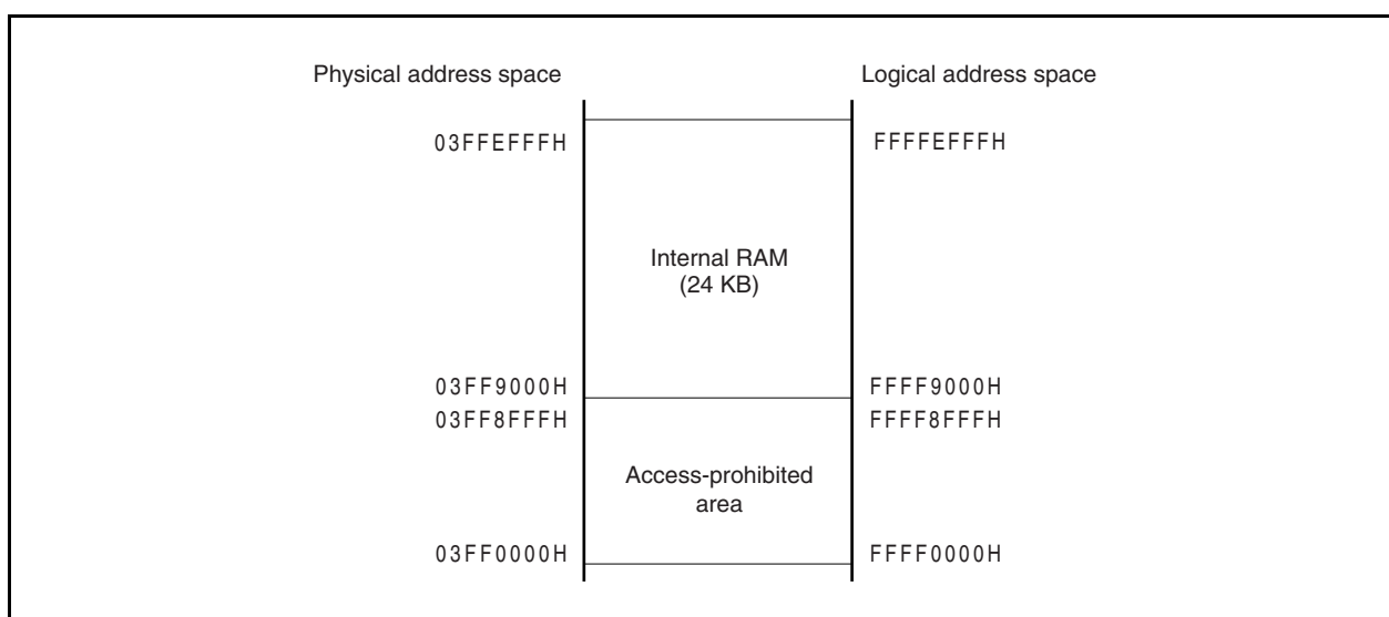
Figure 3-11. Internal RAM Area (24 KB)
