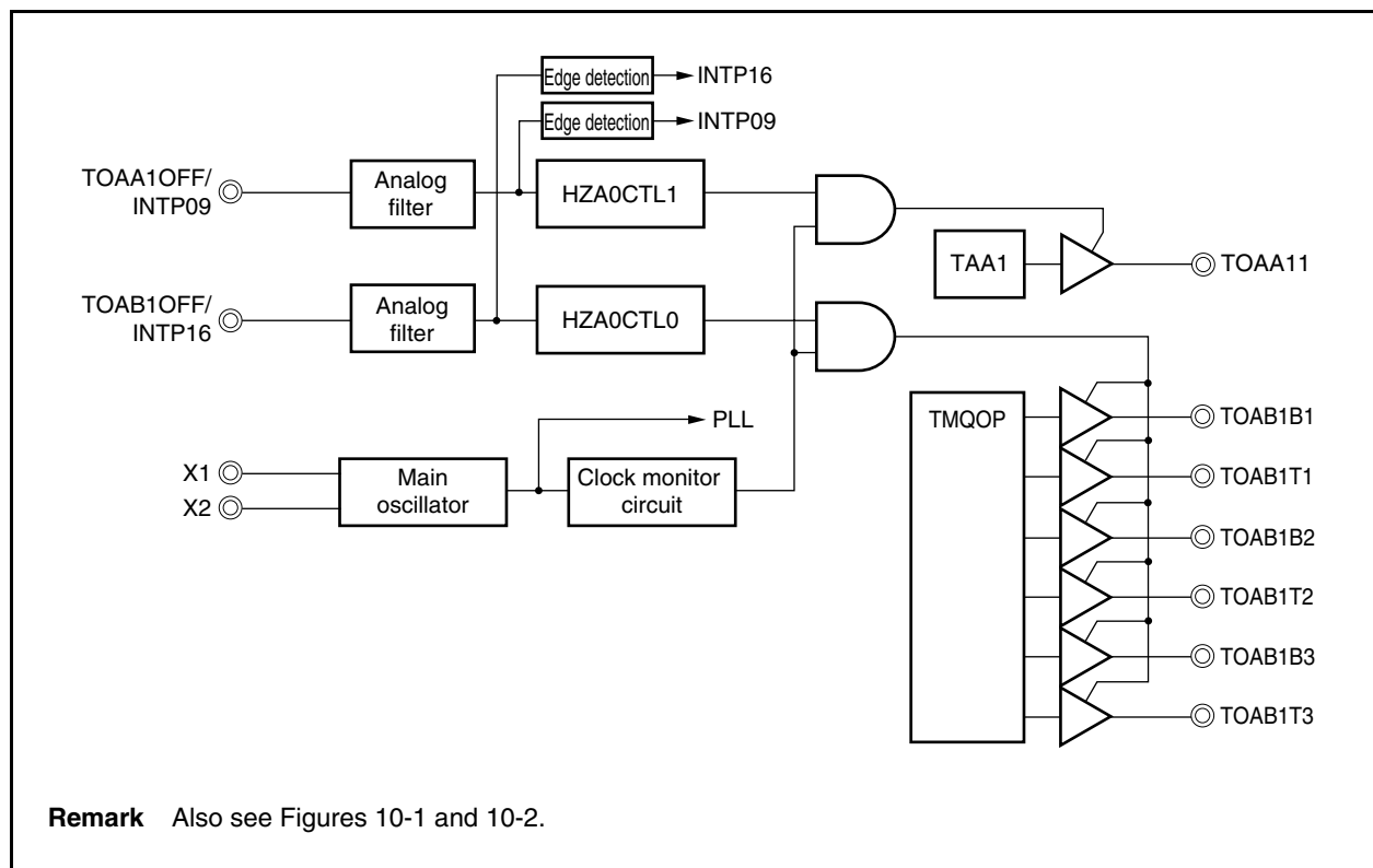
Figure 10-4. High-Impedance Output Controller Configuration
