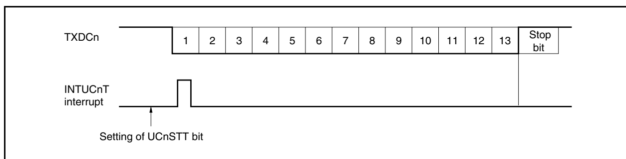
Figure 16-9. SBF Transmission
