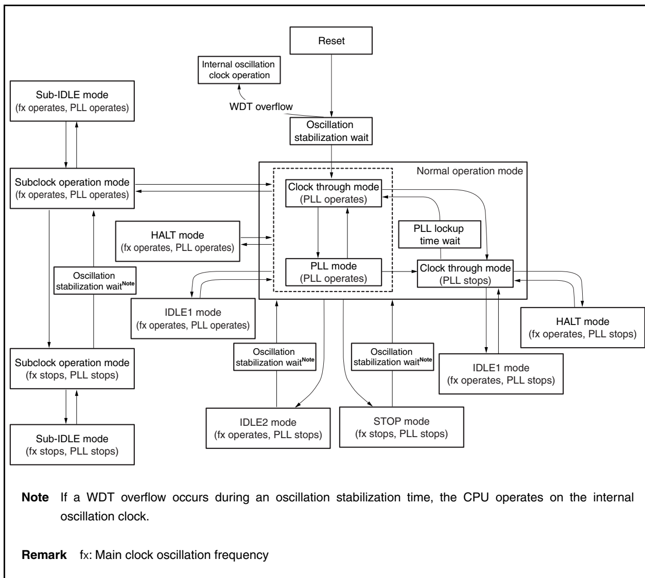
Figure 24-1. Status Transition
