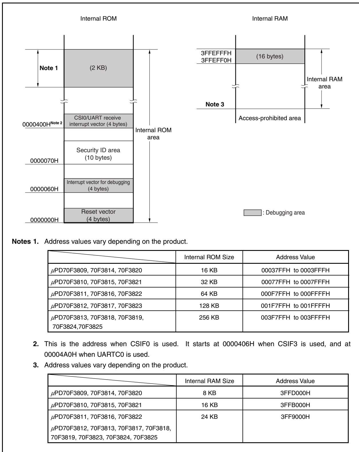
Figure 31-4. Memory Spaces Where Debug Monitor Programs Are Allocated
