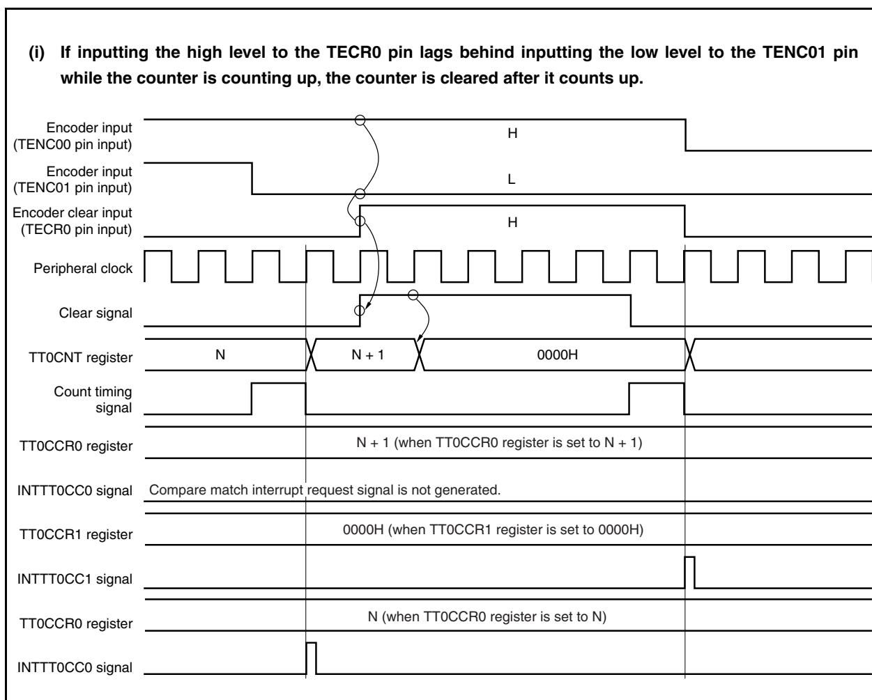
Figure 8-54. Operation Example (When TT0SCE Bit = 1, TT0ZCL Bit = 1, TT0BCL Bit = 0, TT0ACL Bit = 1, TT0UDS1 and TT0UDS0 Bits = 11, TECR0 = High Level, TENC01 = Low Level, and TENC00 = High Level) (1/3)
