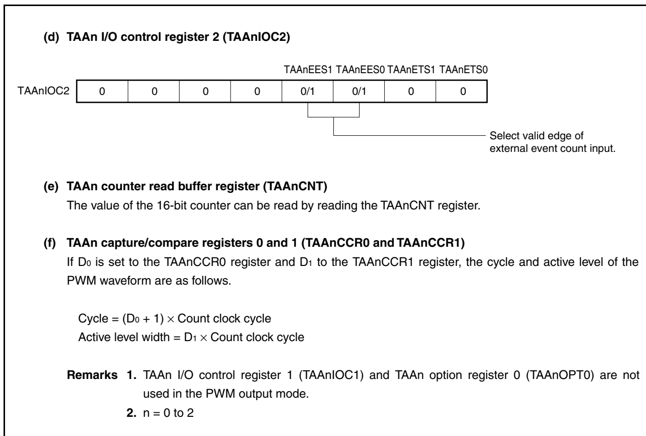
Figure 6-31. Setting of Registers in PWM Output Mode (2/2)
