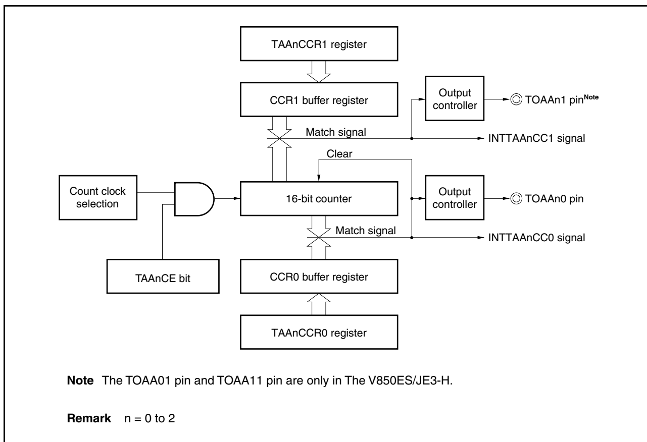
Figure 6-11. Configuration of TAA n CCR1 Register
