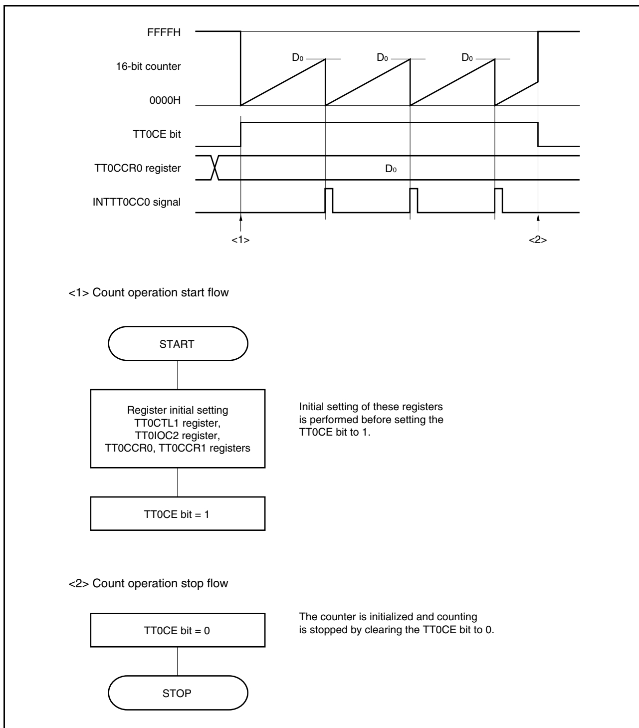
Figure 8-17. Software Processing Flow in External Event Count Mode
