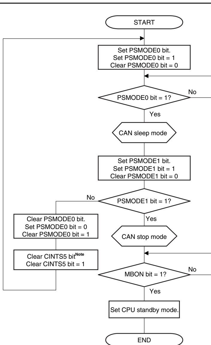
Figure 19-60. Setting CPU Standby (from CAN Stop Mode)
