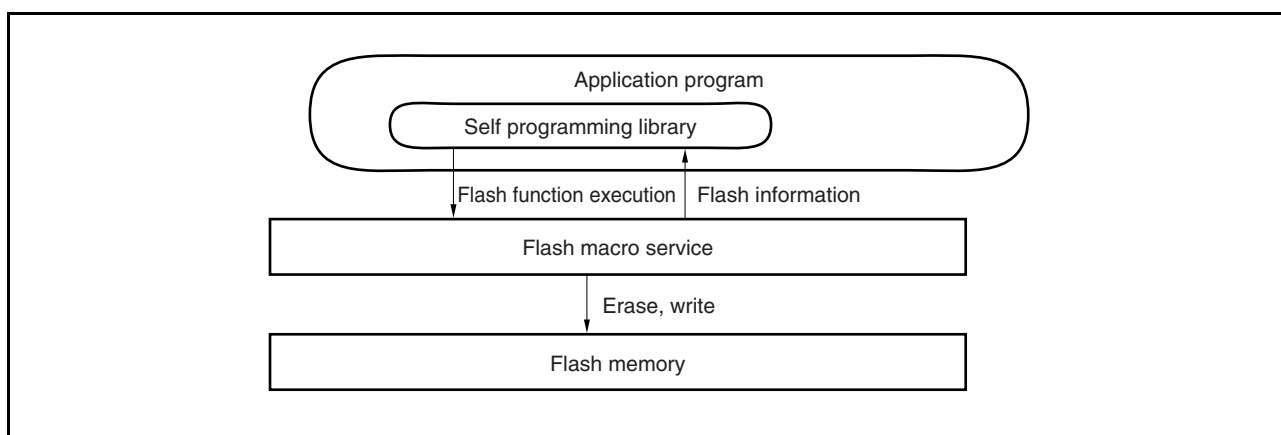
Figure 30-17. Concept of Self Programming
