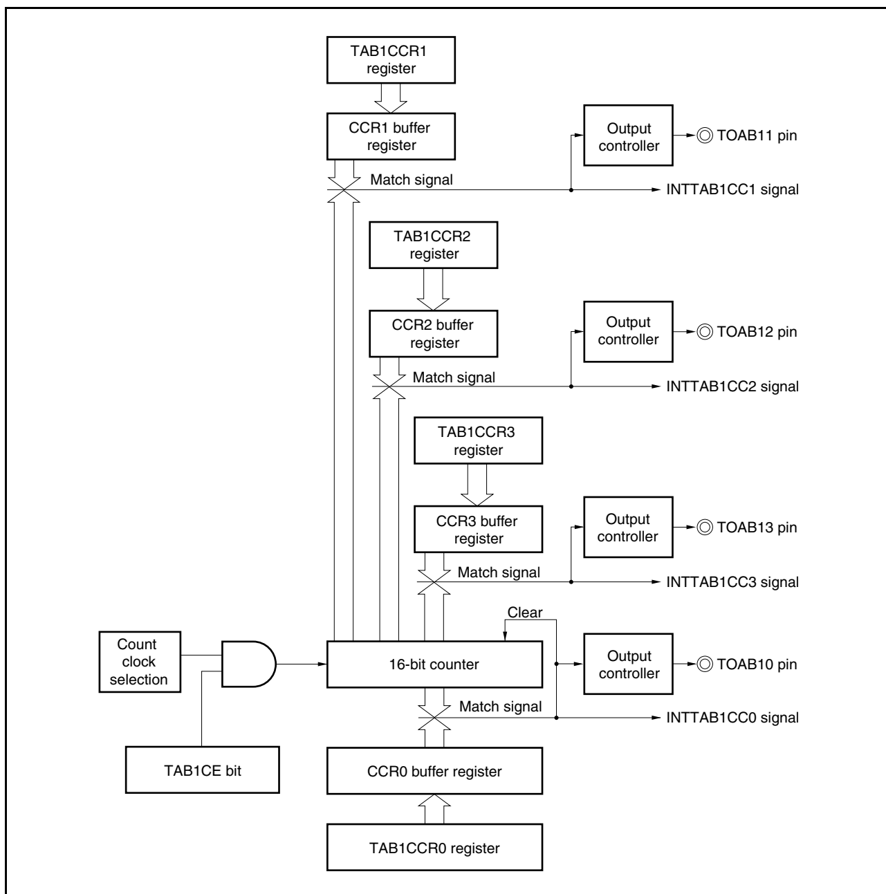
Figure 7-6. Configuration of TAB1CCR1 to TAB1CCR3 Registers
