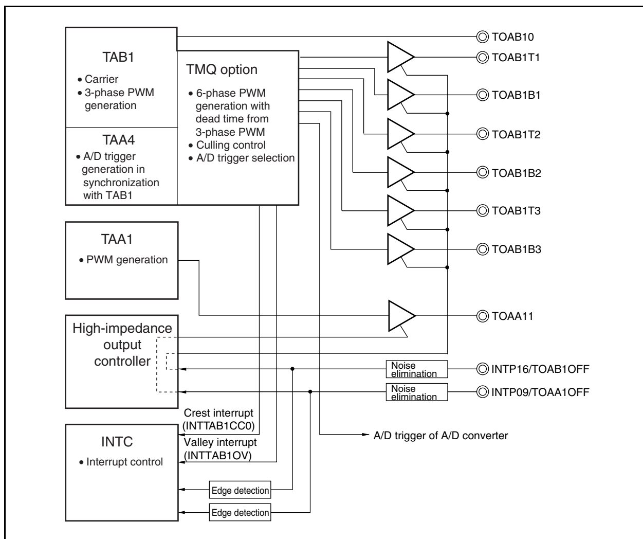
Figure 10-1. Block Diagram of Motor Control
