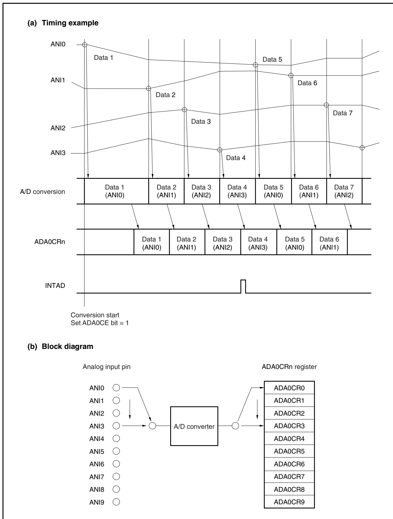
Figure 14-5. Timing Example of Continuous Scan Mode Operation (ADA0S Register = 03H)
