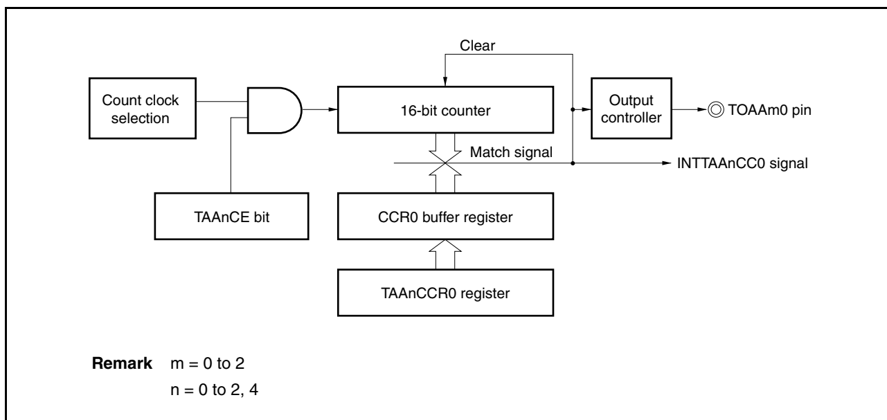
Figure 6-7. Configuration of Interval Timer
