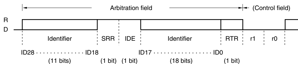
Figure 19-7. Arbitration Field (in Extended Format Mode)
