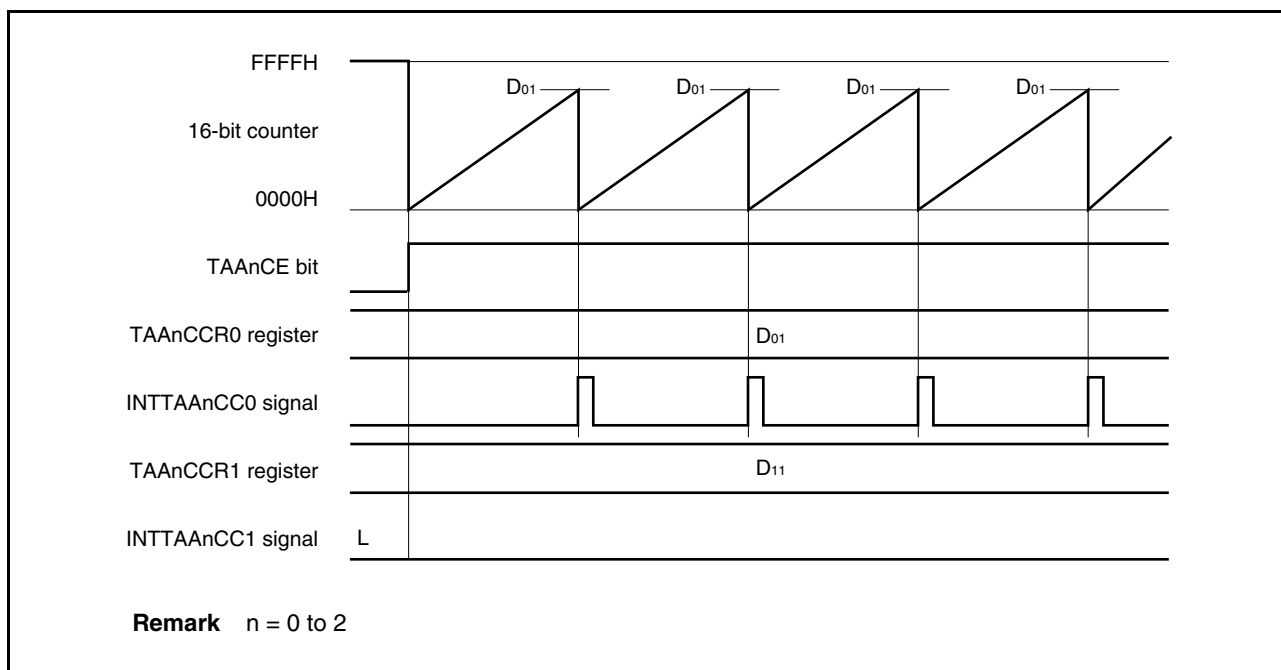
Figure 6-20. Timing Chart When D_{01} < D_{11}
