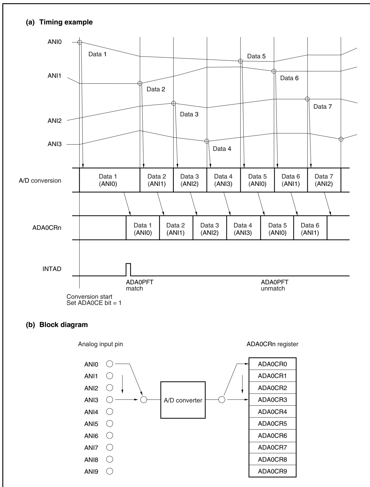
Figure 14-9. Timing Example of Continuous Scan Mode Operation (When Power-Fail Comparison Is Made: ADA0S Register = 03H)
