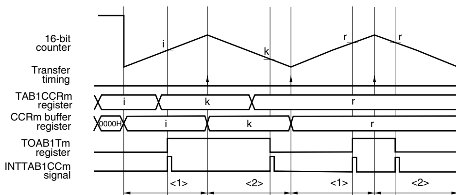
Figure 10-30. Example of Rewriting TAB1CCRm Register
