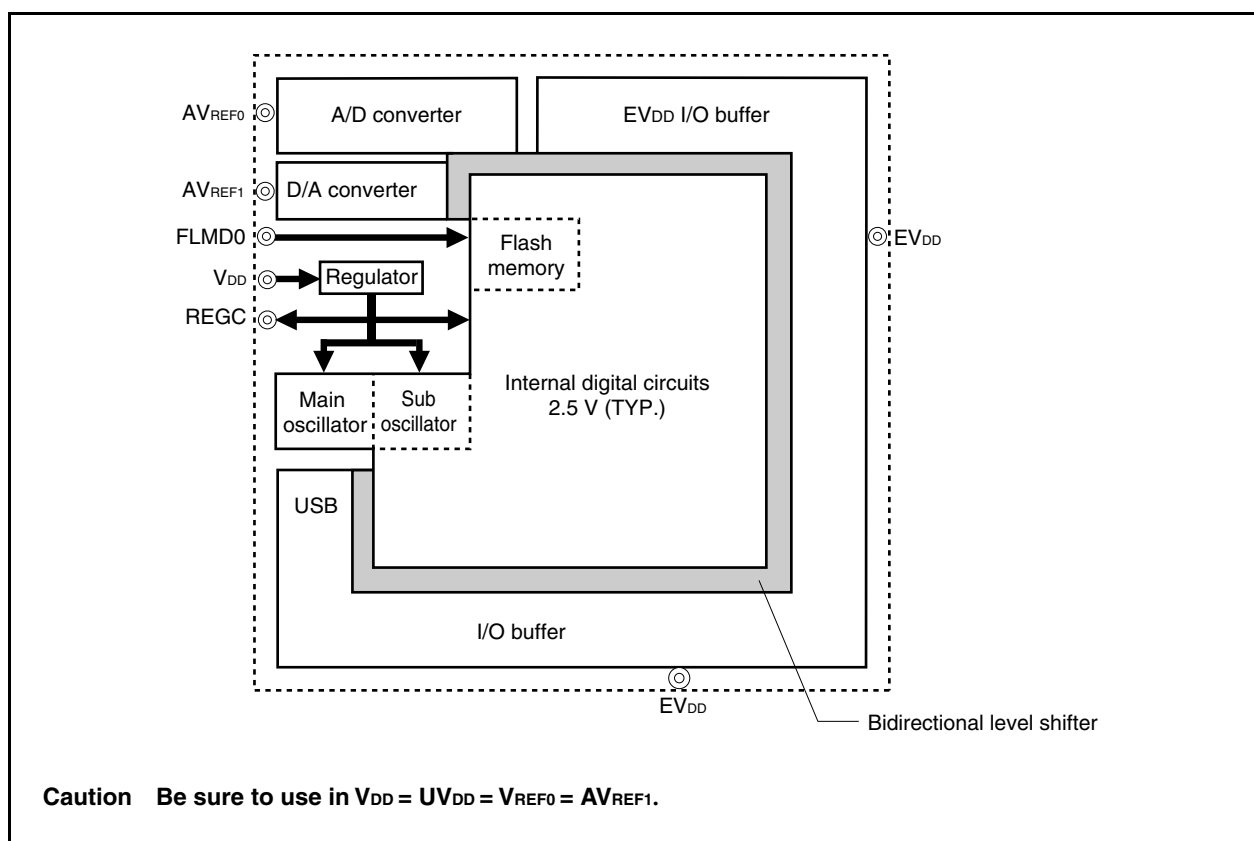
Figure 29-1. Regulator
