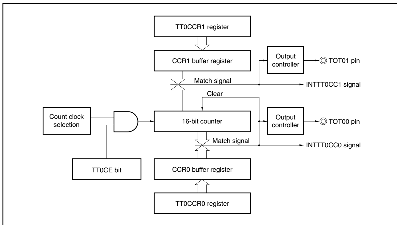
Figure 8-11. Configuration of TT0CCR1 Register
