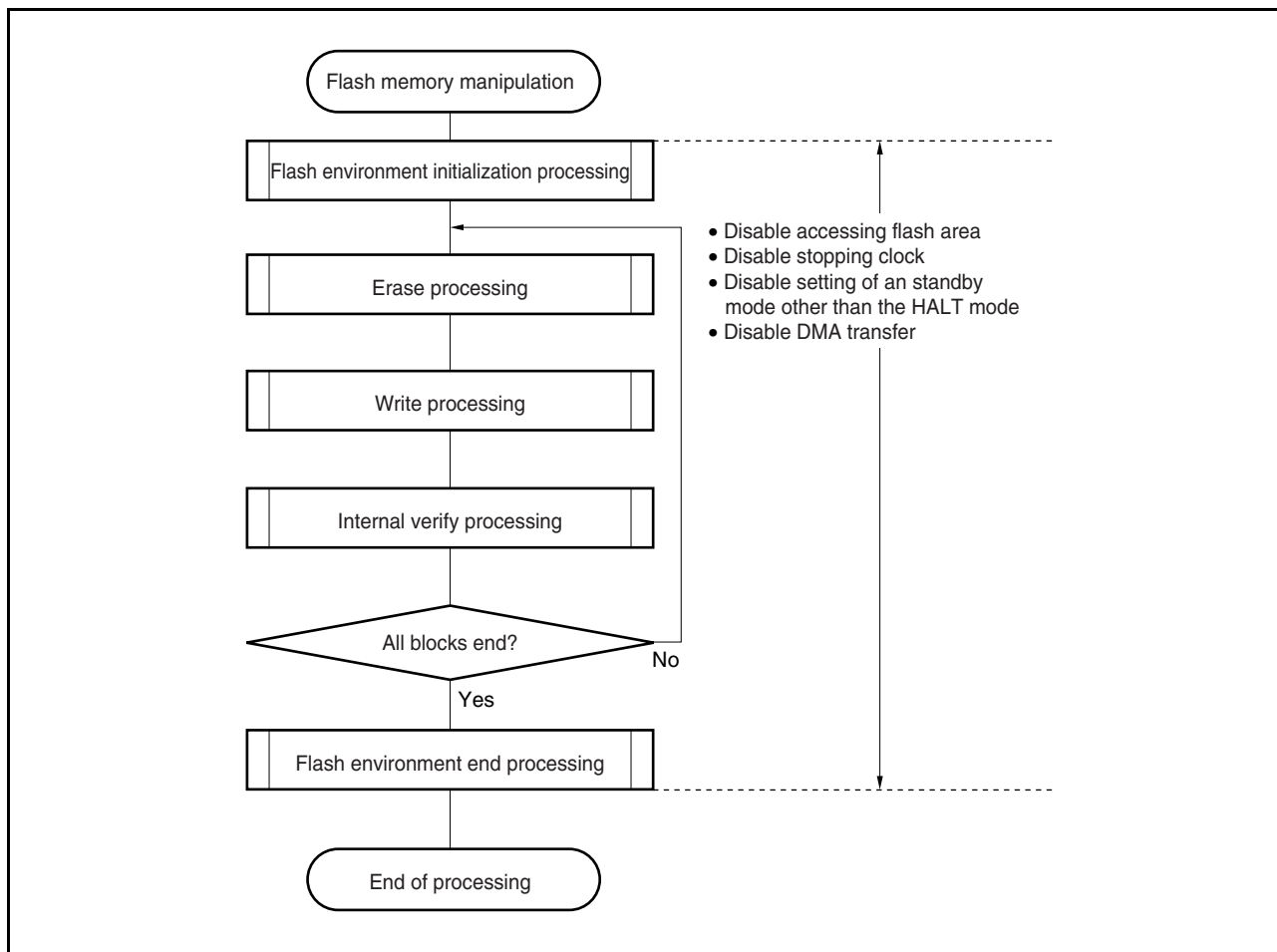
Figure 30-19. Standard Self Programming Flow
