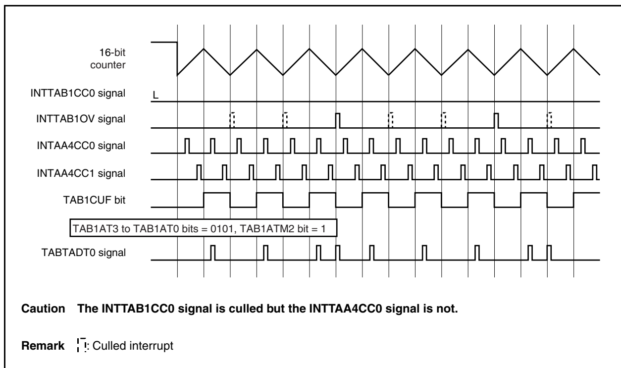
Figure 10-40. Example of A/D Conversion Start Trigger (TABTADT0) Signal Output (TAB1OPT1.TAB1ICE Bit = 0, TAB1OPT1.TAB1IOE Bit = 1, TAB1OPT1.TAB1ID4 to TAB1OPT1.TAB1ID0 Bits = 00010: With Interrupt Culling) (2)
