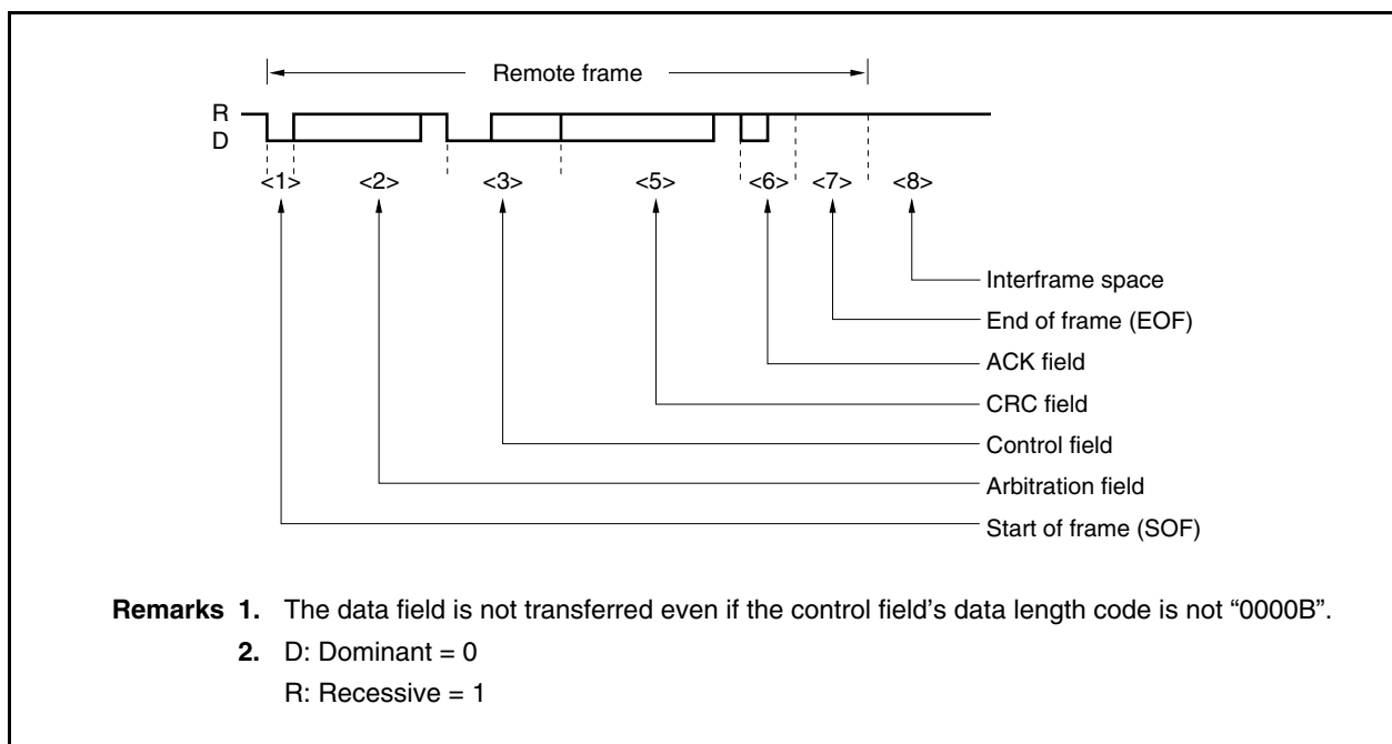
Figure 19-4. Remote Frame
