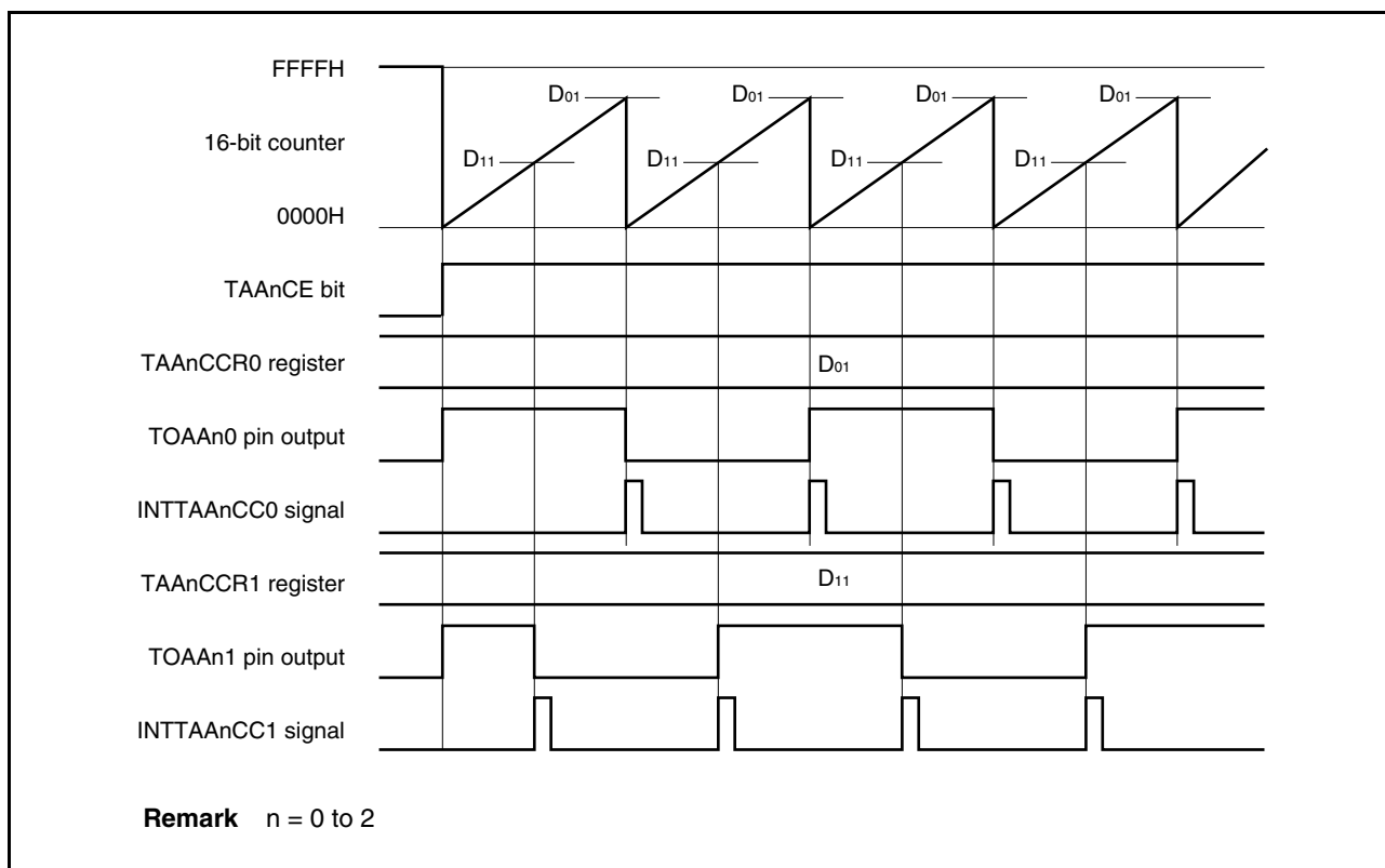
Figure 6-12. Timing Chart When D_{01} \geq D_{11}
