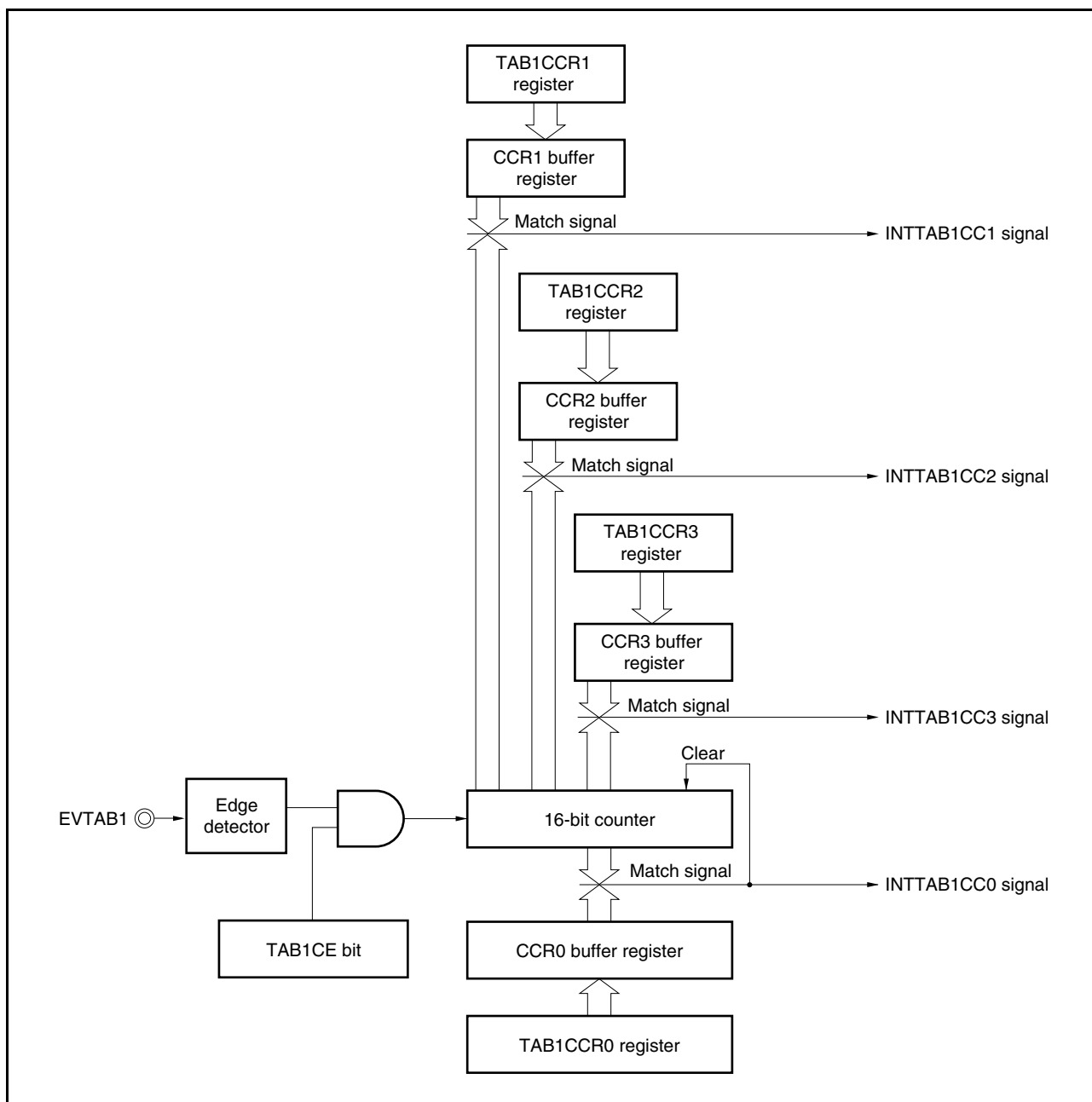
Figure 7-13. Configuration of TAB1CCR1 to TAB1CCR3 Registers
