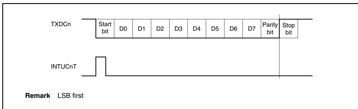
Figure 16-11. UART Transmission
