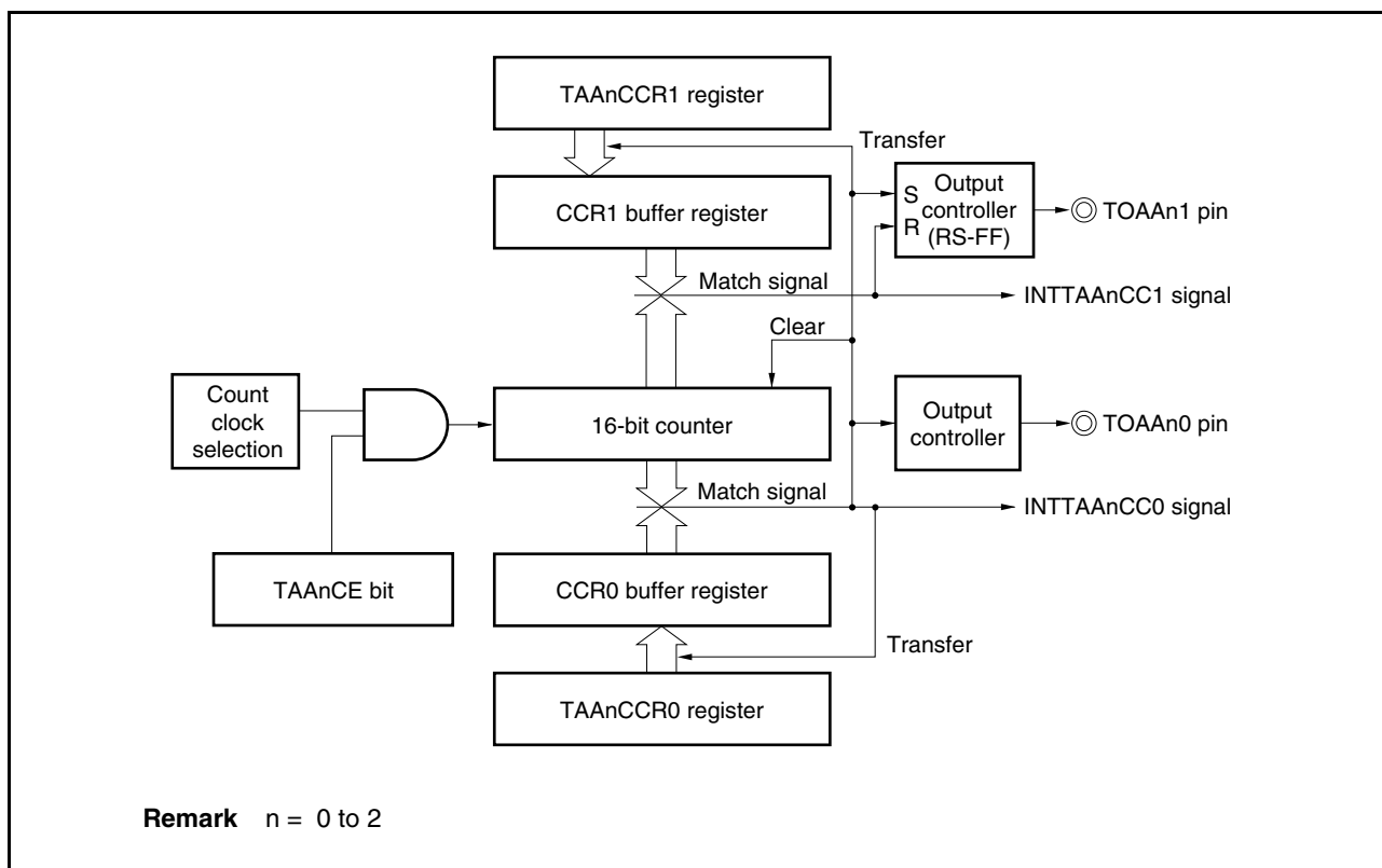
Figure 6-29. Configuration in PWM Output Mode
