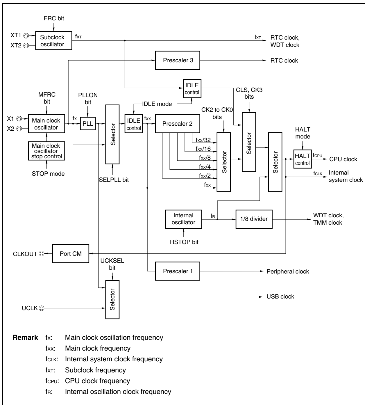
Figure 5-1. Clock Generator
