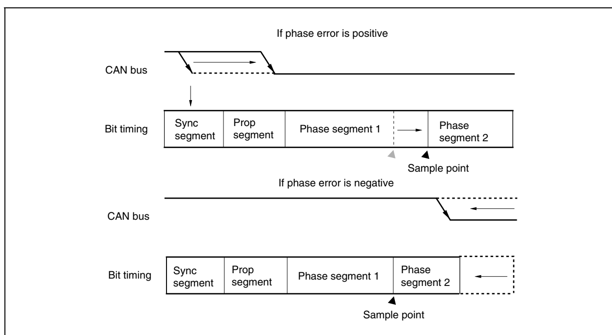
Figure 19-21. Resynchronization
