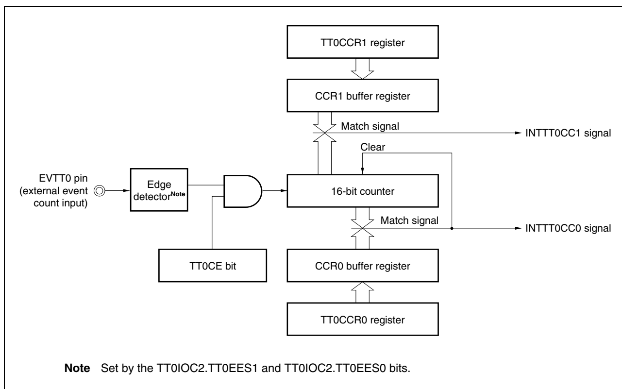
Figure 8-18. Configuration of TT0CCR1 Register
