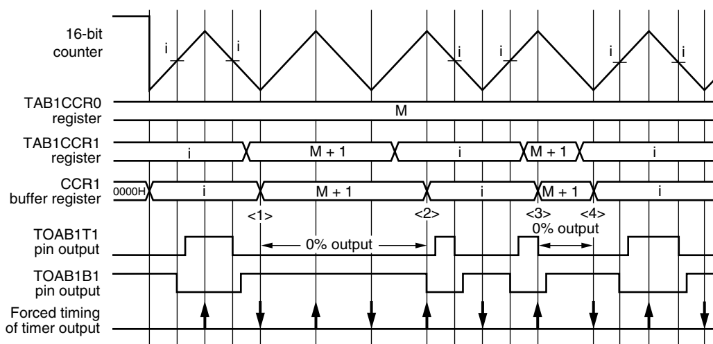
Figure 10-9. 0% PWM Output Waveform (With Dead Time)
