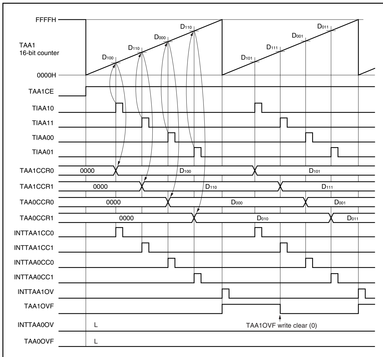
Figure 6-45. Example of Timing in Free-Running Mode (Capture Function)
