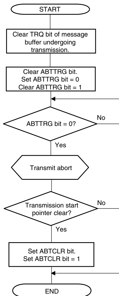
Figure 19-48 (b). ABT Transmission Abort Processing (Normal Operation Mode with ABT)
