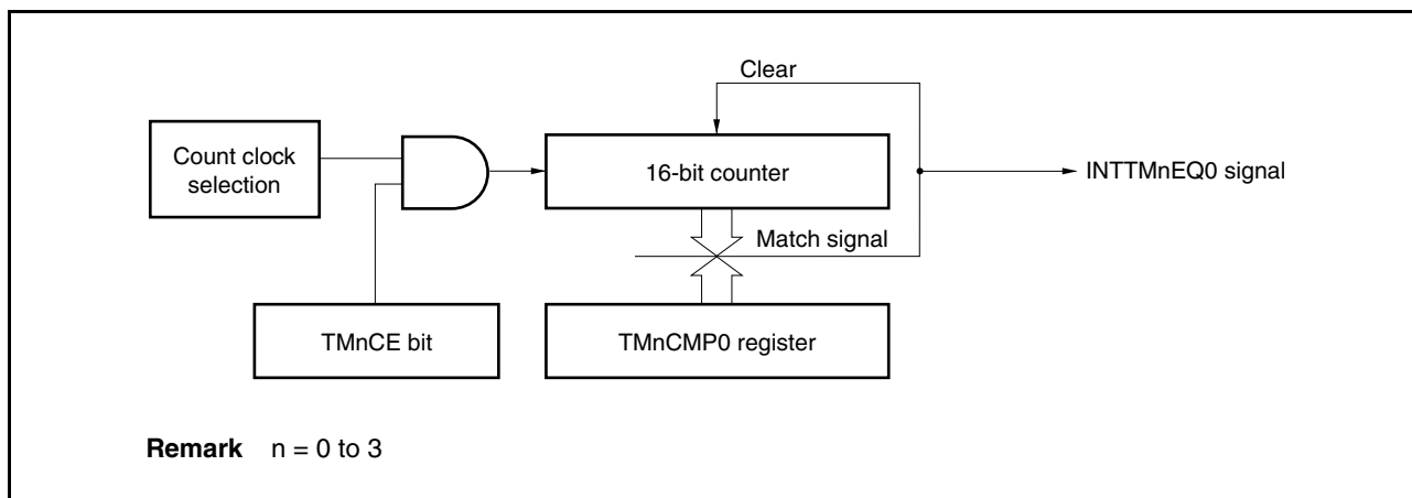
Figure 9-2. Configuration of Interval Timer
