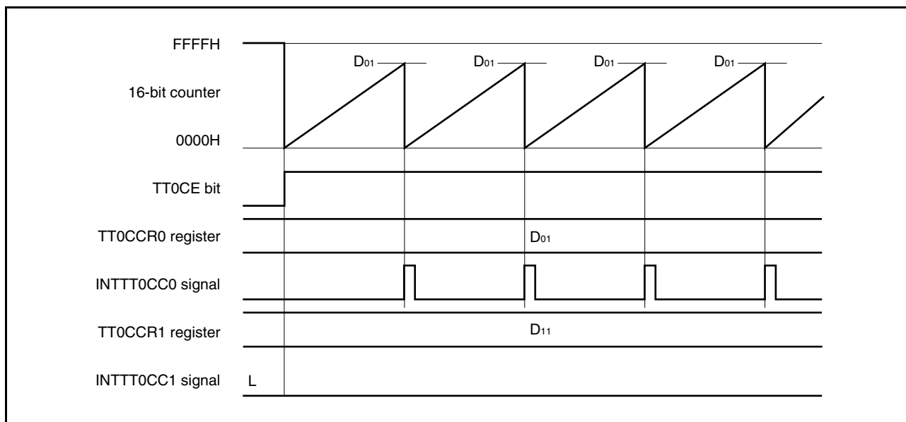
Figure 8-20. Timing Chart When D_{01} < D_{11}
