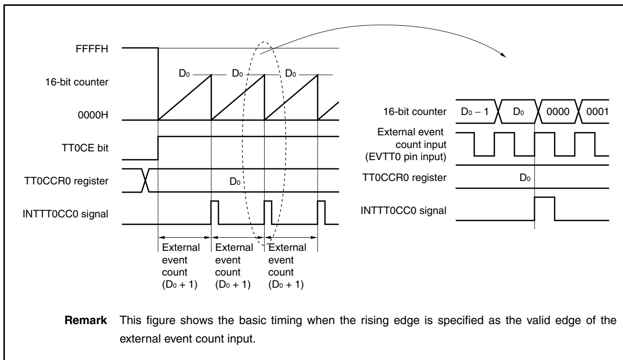
Figure 8-15. Basic Timing in External Event Count Mode
