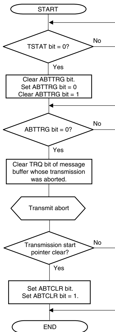
Figure 19-48 (a). ABT Transmission Abort Processing (Normal Operation Mode with ABT)
