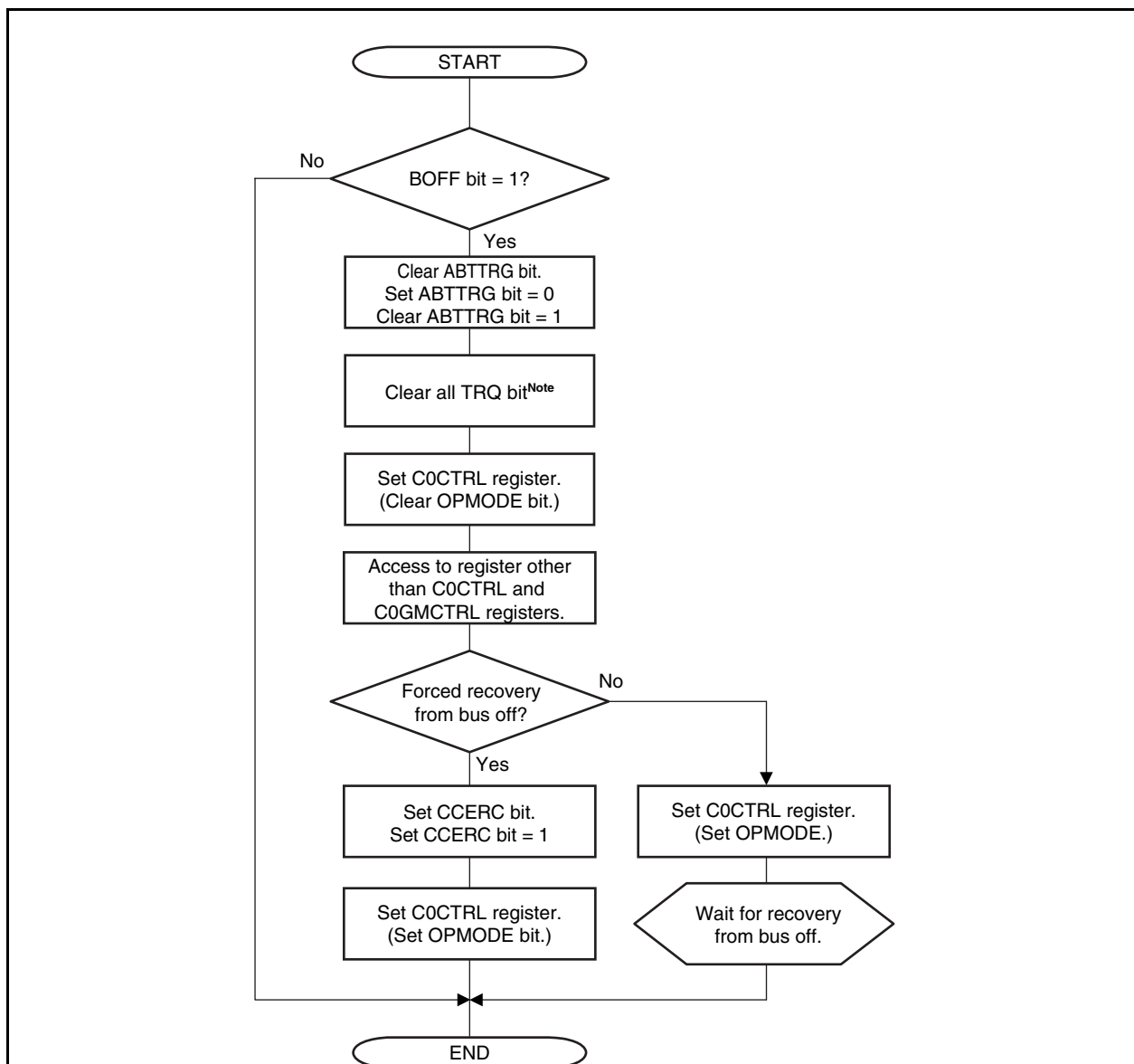
Figure 19-55. Bus-off Recovery (Normal Operation Mode with ABT)
