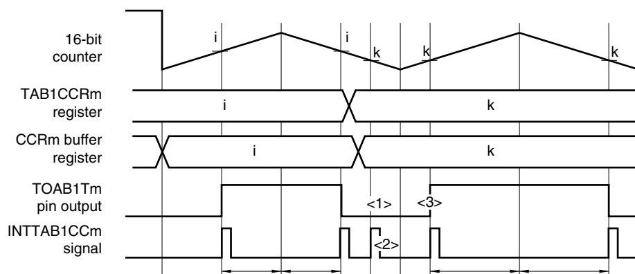
Figure 10-25. Example of Rewriting TAB1CCR1 to TAB1CCR3 Registers (Rewriting After Match Occurs)
