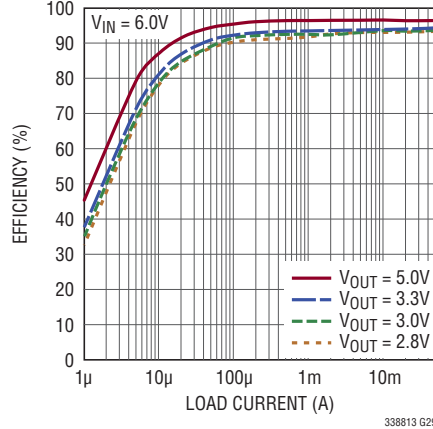
Efficiency vs I_{LOAD} , L = 100\mu H (LTC3388-3)
