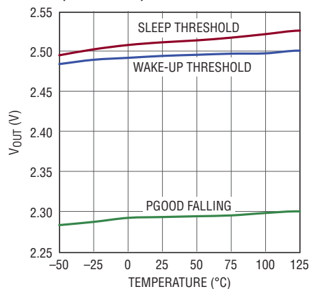
2.5V Output vs Temperature (LTC3388-1)
