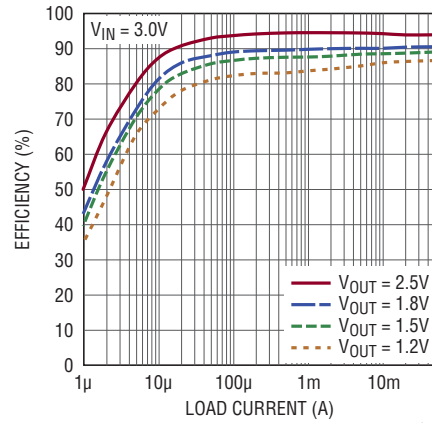
Efficiency vs I_{LOAD} , L = 100\mu H (LTC3388-1)
