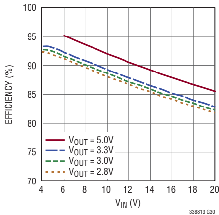
Efficiency vs V_{IN} for I_{LOAD} = 50mA , L = 22\mu H (LTC3388-3)
