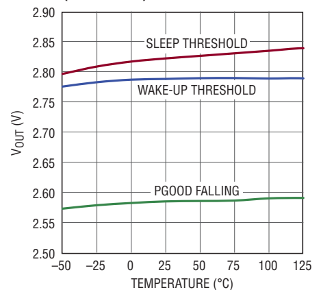
2.8V Output vs Temperature (LTC3388-3)
