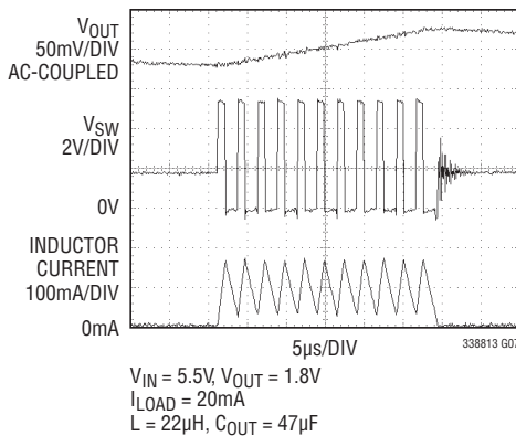
Operating Waveforms
