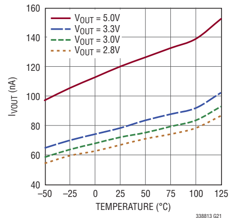
I OUT vs Temperature (LTC3388-3)
