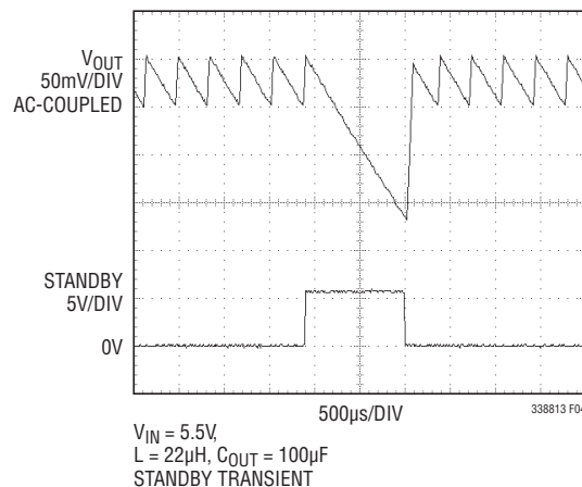
Figure 4. LTC3388-3 Standby Transient, V_{OUT} = 3.3V , I_{LOAD} = 5mA
