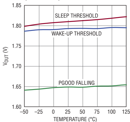
1.8V Output vs Temperature (LTC3388-1)
