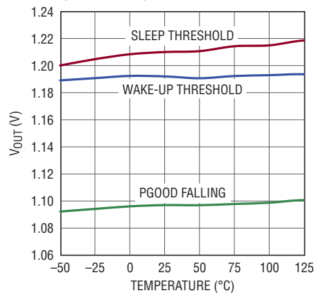
1.2V Output vs Temperature (LTC3388-1)
