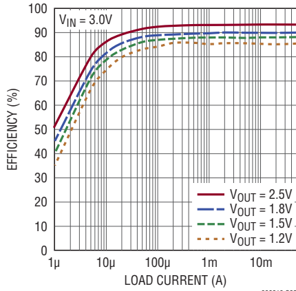
Efficiency vs I_{LOAD} , L = 22\mu H (LTC3388-1)
