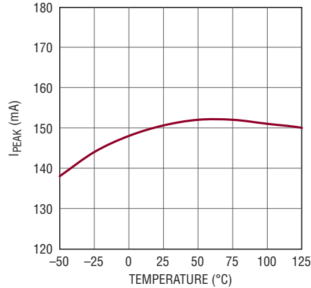
I_{PEAK} vs Temperature
