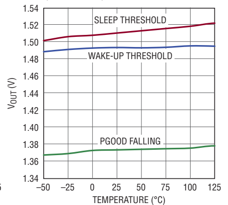
1.5V Output vs Temperature (LTC3388-1)
