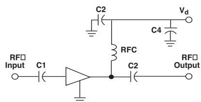
Figure 15. Schematic Diagram.
