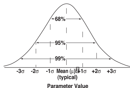
Figure 12. Normal Distribution.
