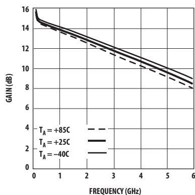
Figure 1. 50 Power Gain vs. Frequency and Temperature.
