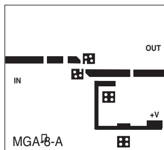
Figure 14. PCB Layout.
