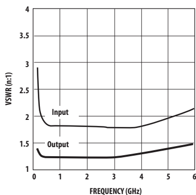
Figure 7. Input and Output VSWR into 50 vs. Frequency.
