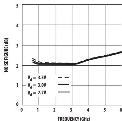
Figure 5. Noise Figure (into 50) vs. Frequency and Voltage.
