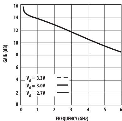
Figure 4. 50 Power Gain vs. Frequency and Voltage.
