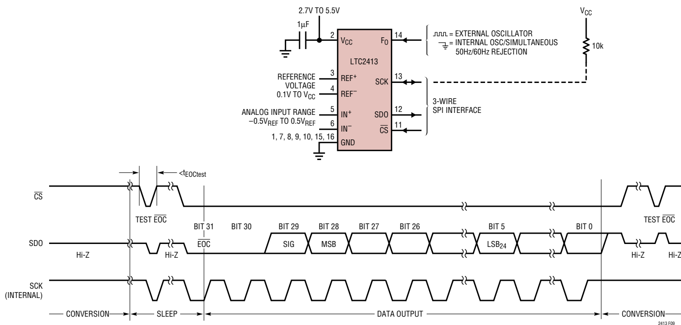
Figure 9. Internal Serial Clock, Single Cycle Operation
