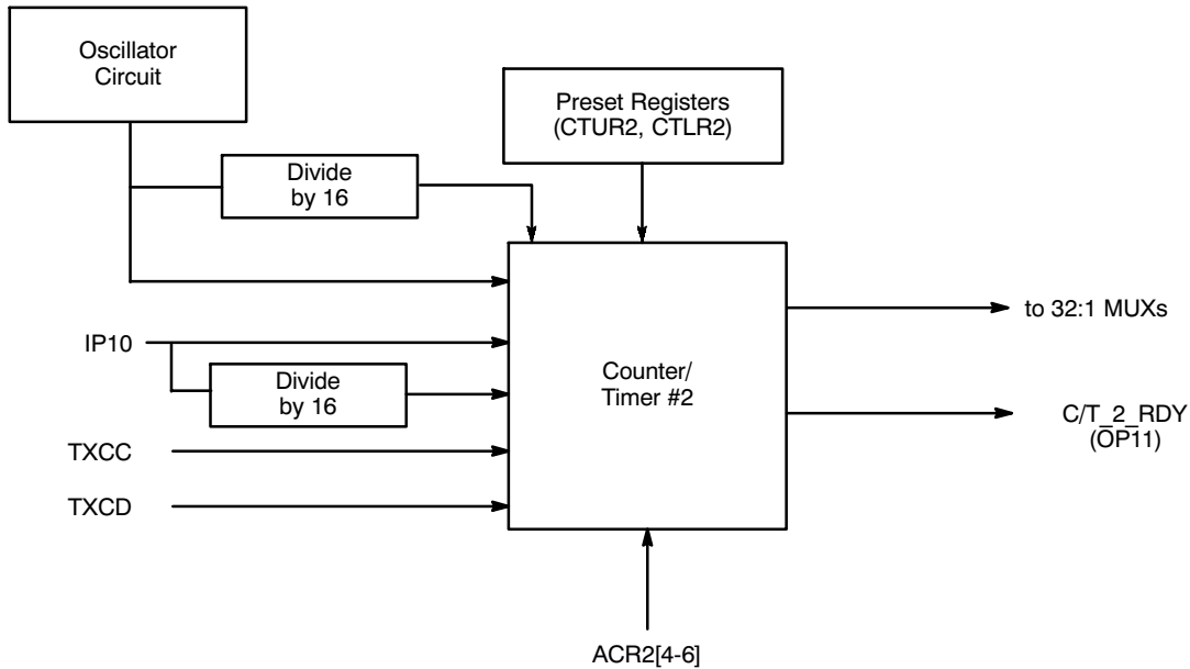
Figure 32A. A Block Diagram of the Circuitry Associated with Counter/Timer #2
